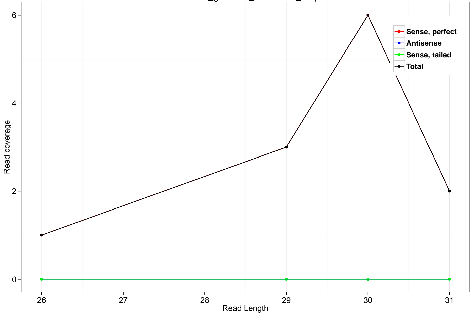
rheMac3_genscan_chr2.1706_9.3p
