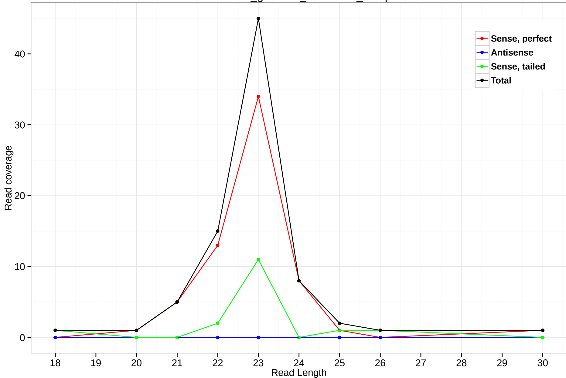
rheMac3_genscan_chr2.1689_38.3p
