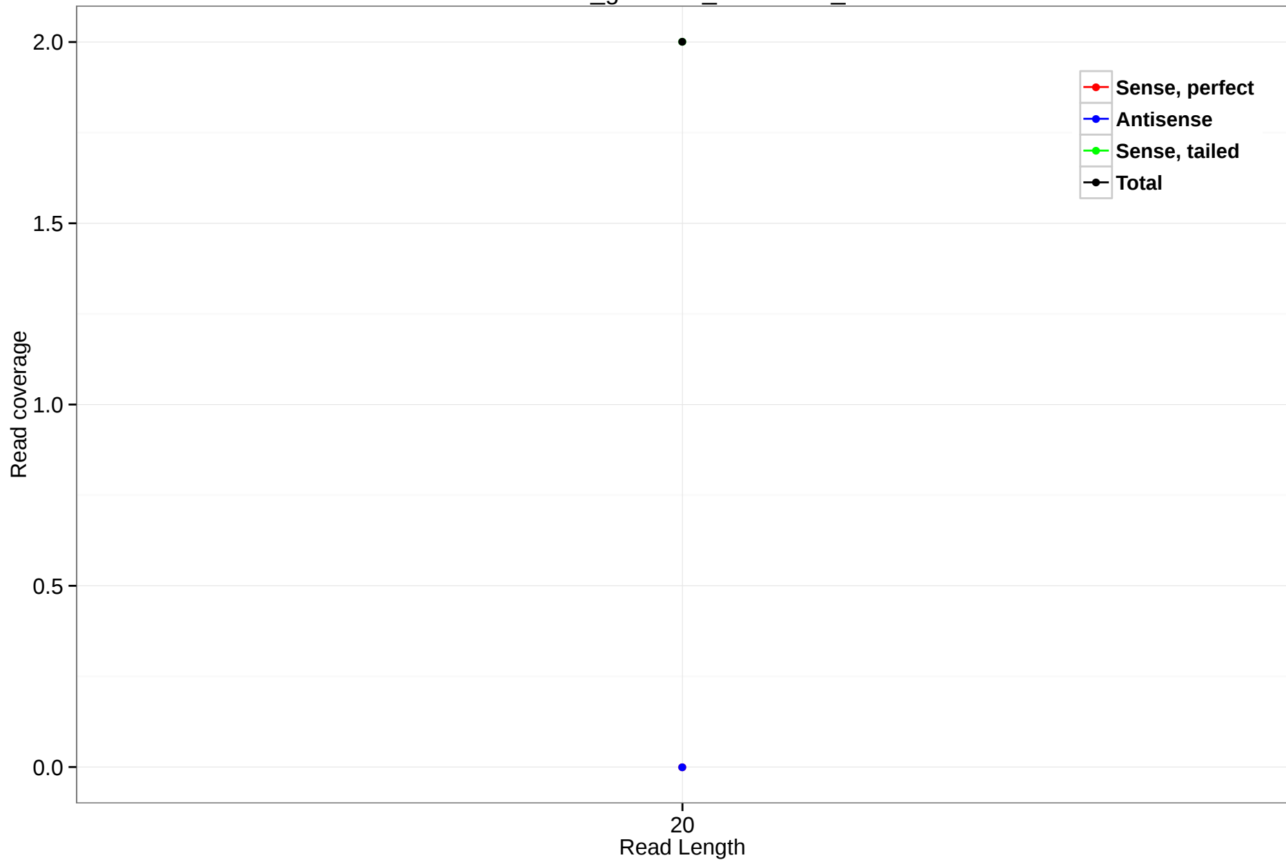
rheMac3_genscan_chr2.1682_23
