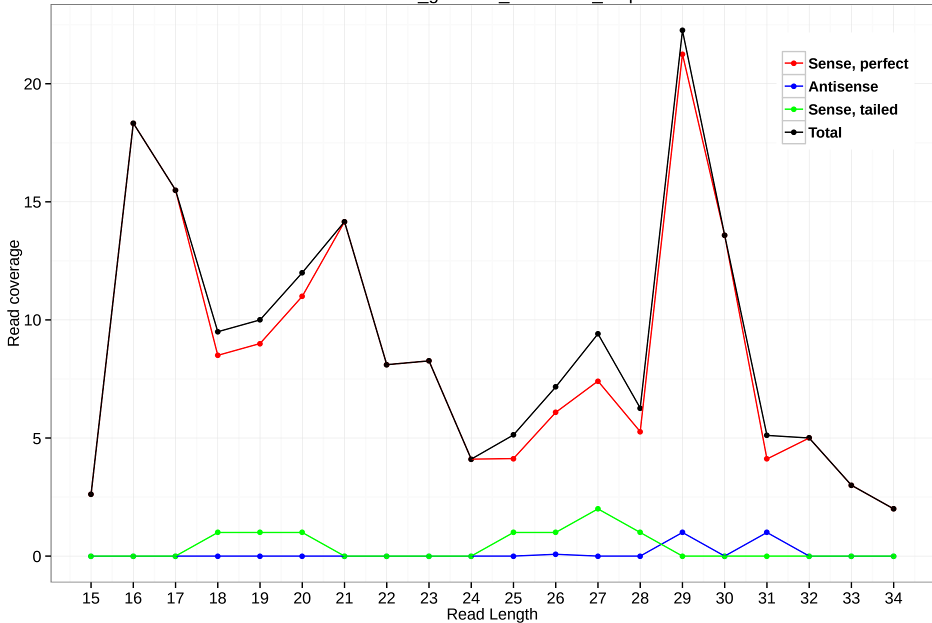
rheMac3_genscan_chr2.1676_8.3p
