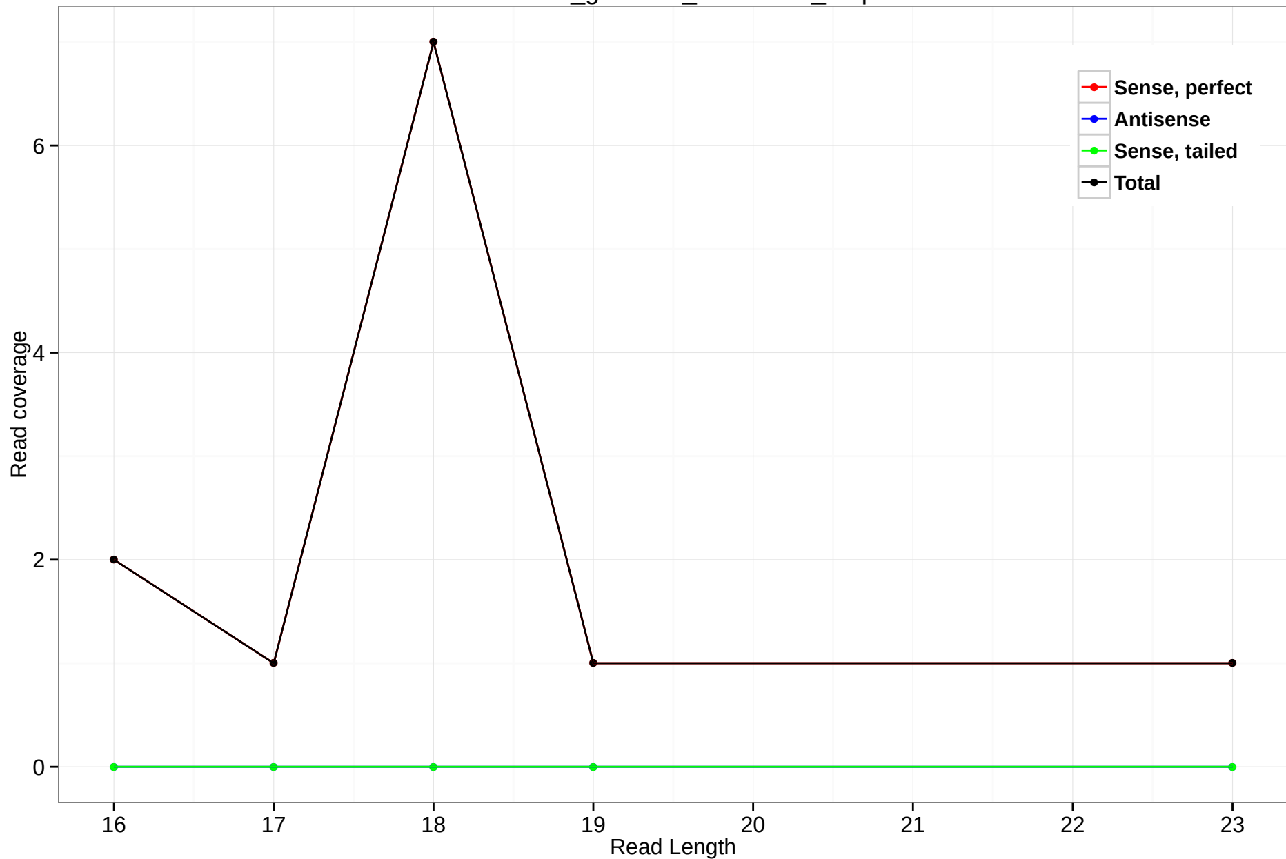
rheMac3_genscan_chr2.1657_4.3p
