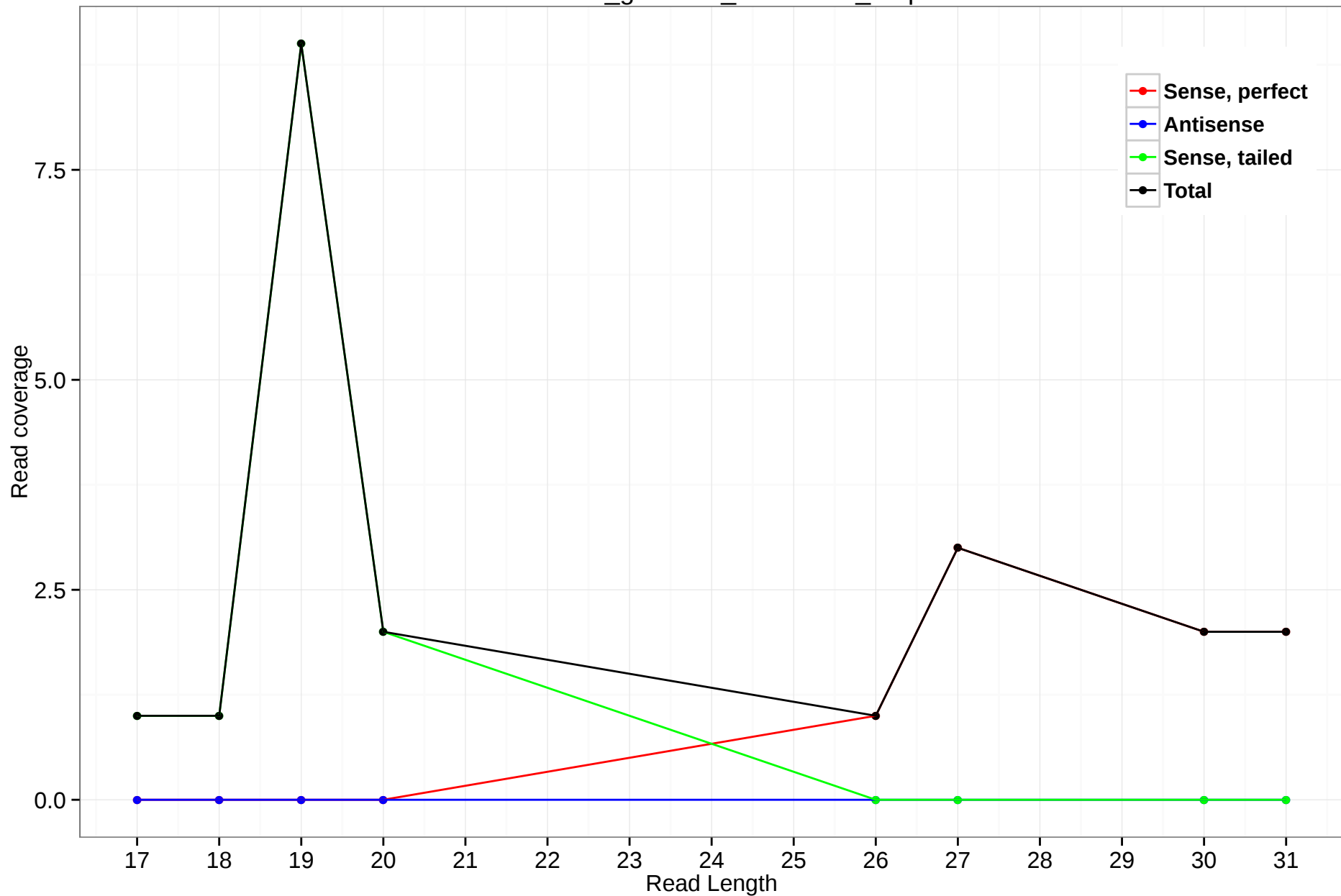
rheMac3_genscan_chr2.1573_1.5p
