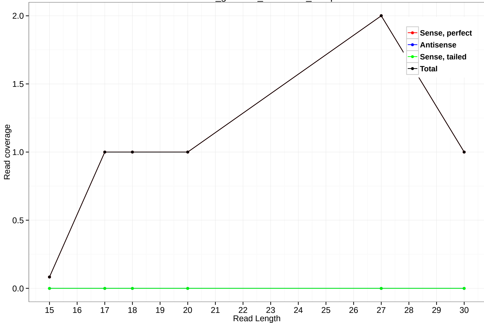
rheMac3_genscan_chr2.1572_23.3p
