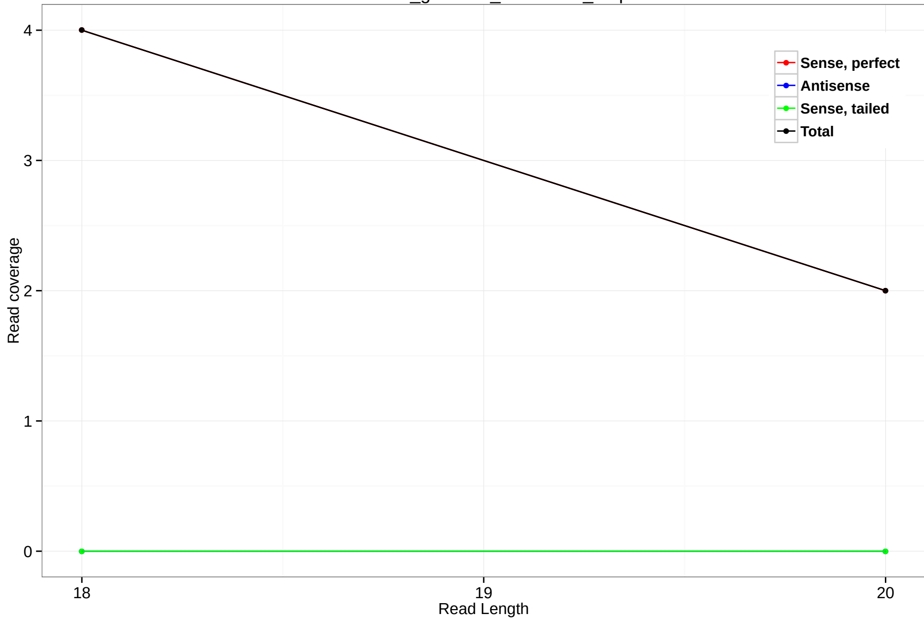
rheMac3_genscan_chr2.1523_2.3p
