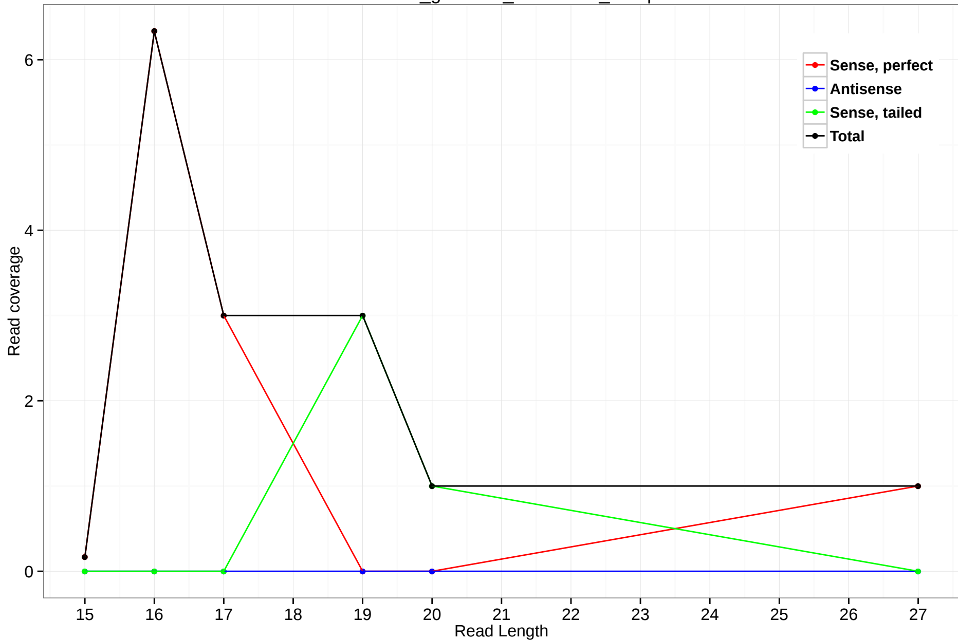
rheMac3_genscan_chr2.1517_11.5p
