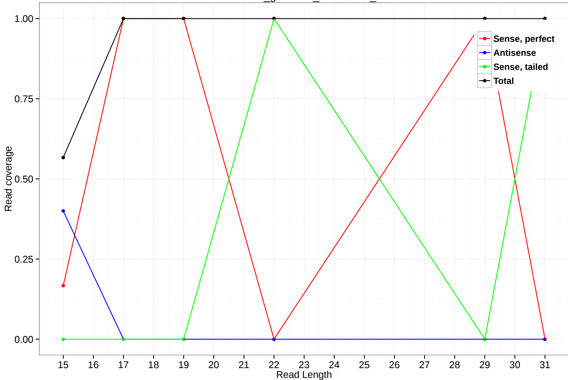
rheMac3_genscan_chr2.1513_26
