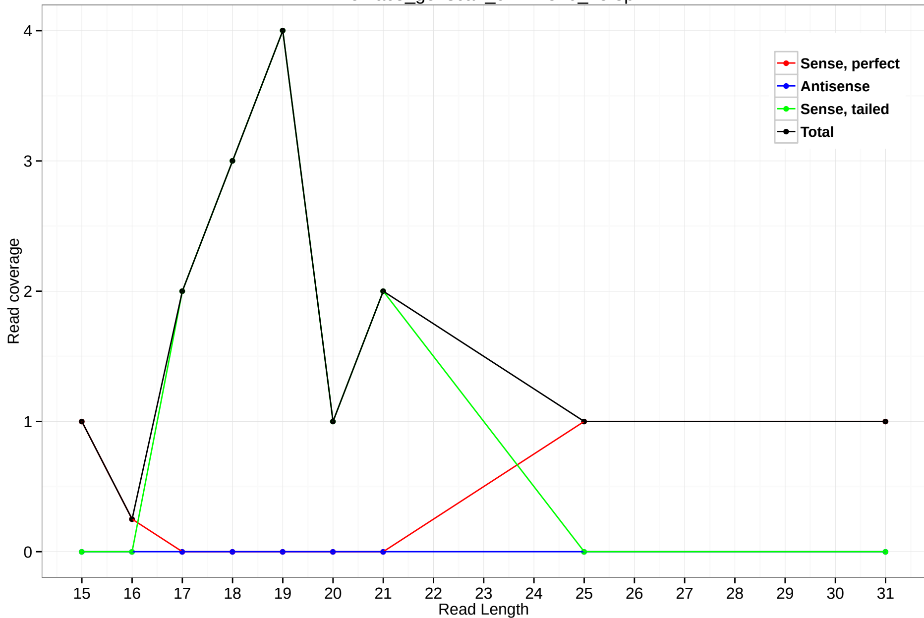
rheMac3_genscan_chr2.1510_18.3p
