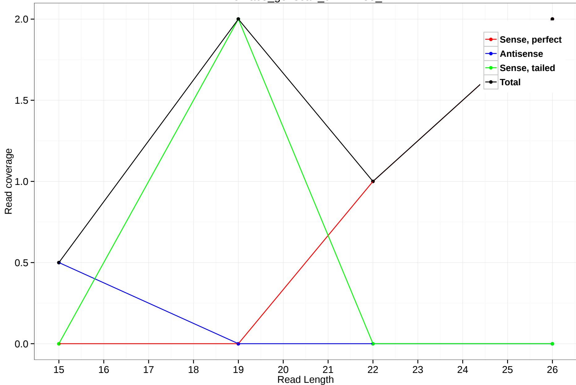
rheMac3_genscan_chr2.1488_2
