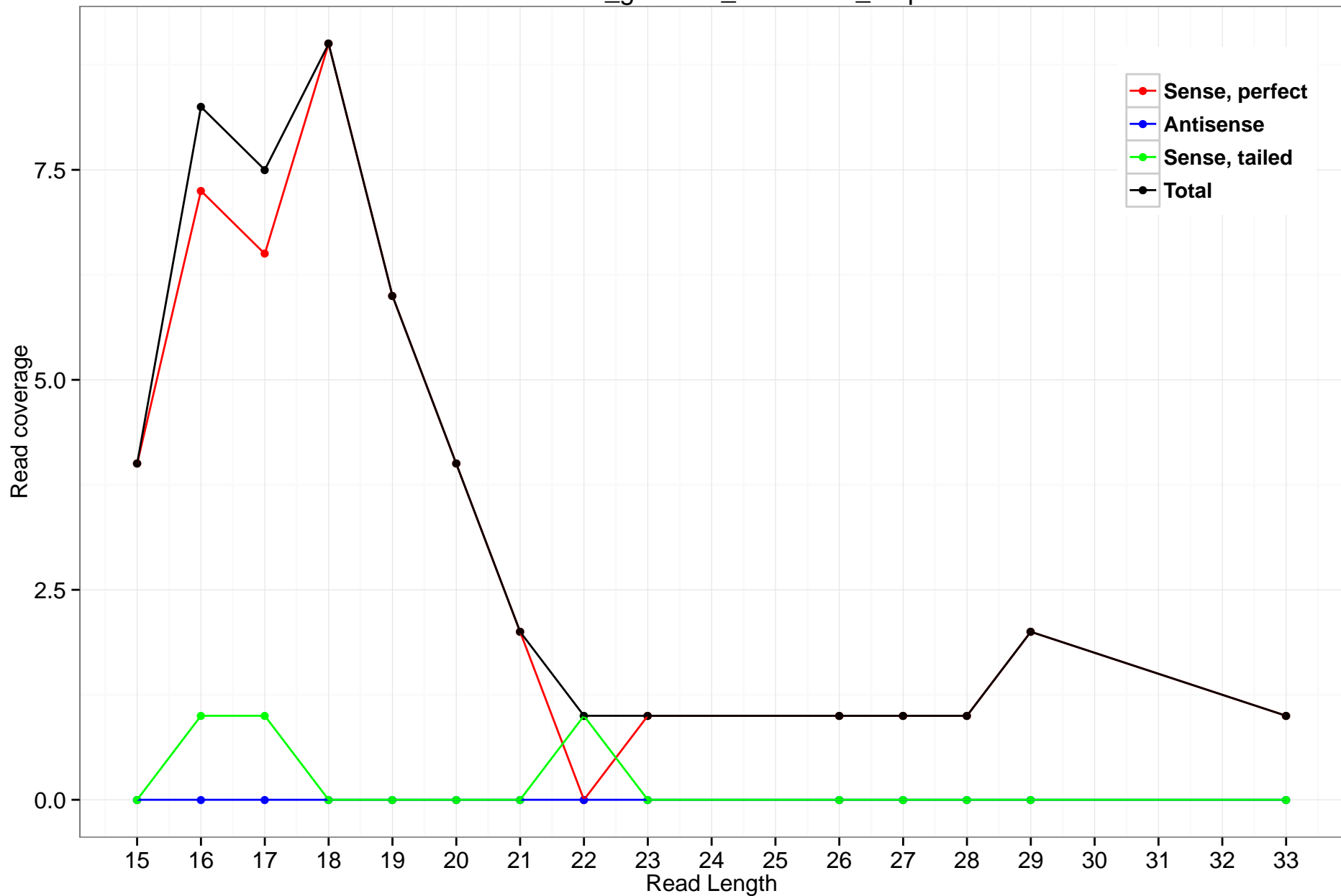
rheMac3_genscan_chr2.1485_1.5p
