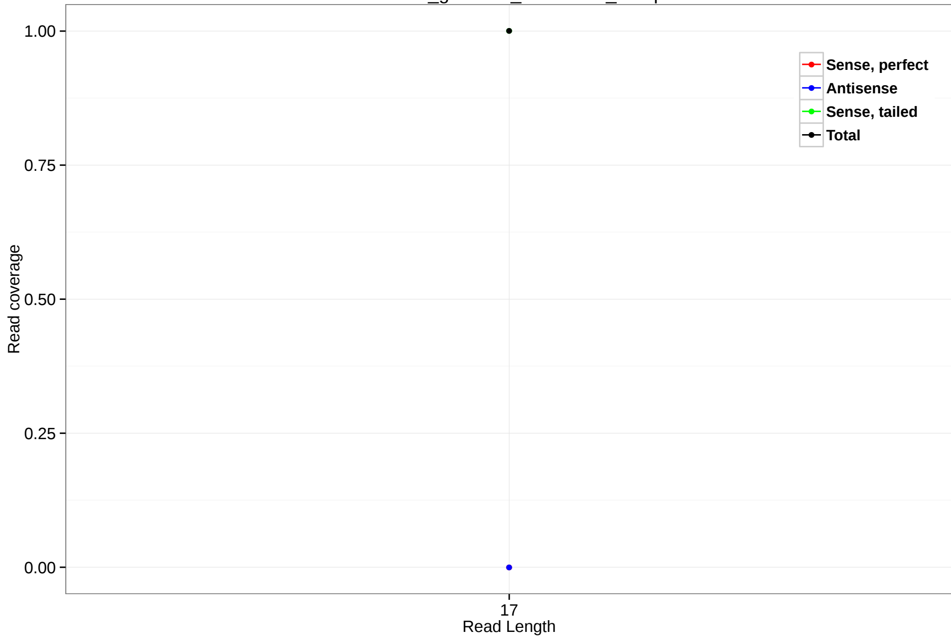
rheMac3_genscan_chr2.1484_27.5p
