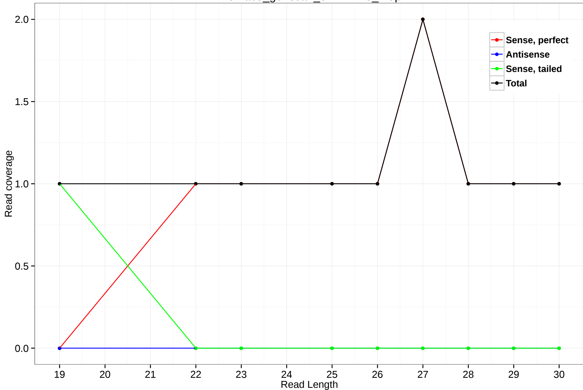
rheMac3_genscan_chr2.1473_1.5p
