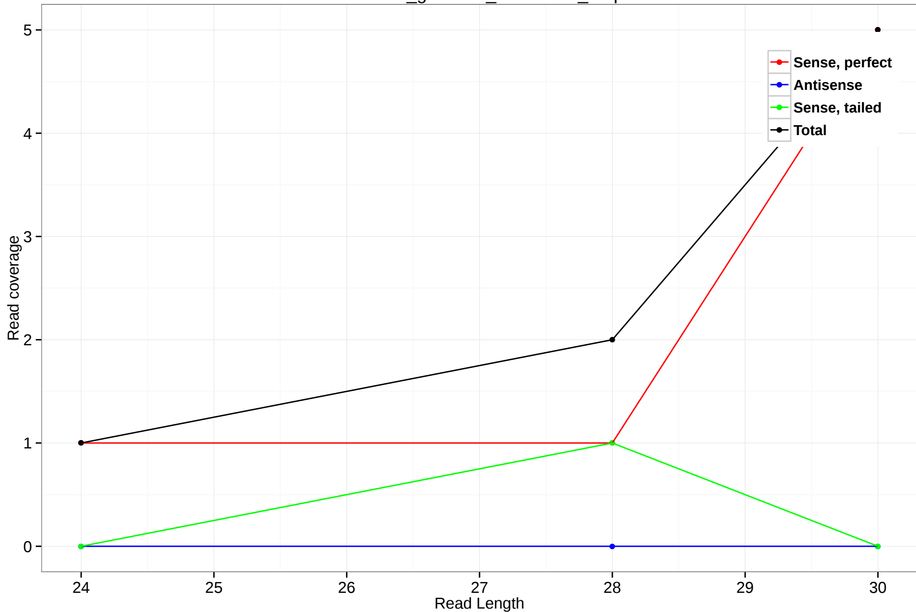
rheMac3_genscan_chr2.1445_1.3p
