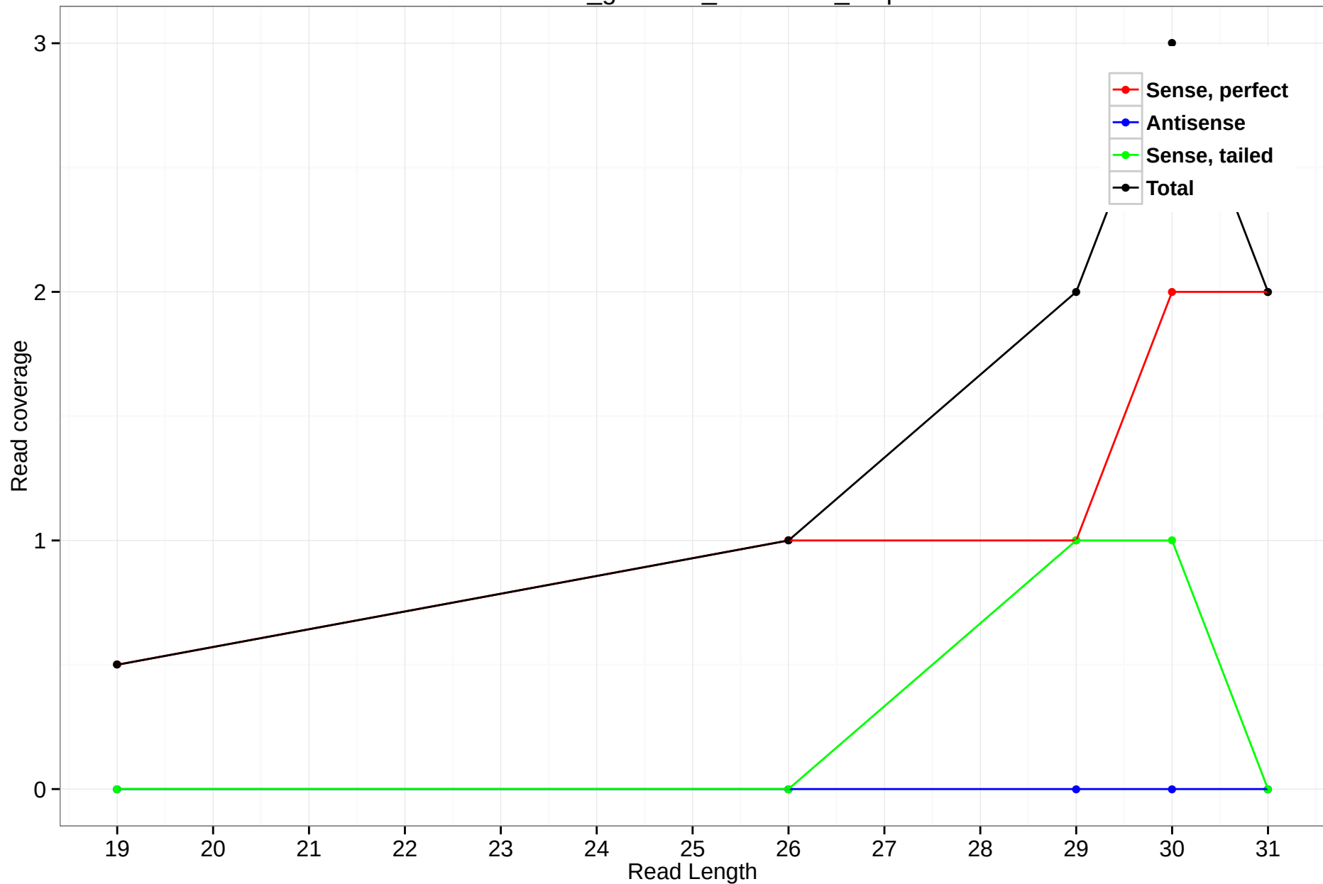
rheMac3_genscan_chr2.1444_4.5p
