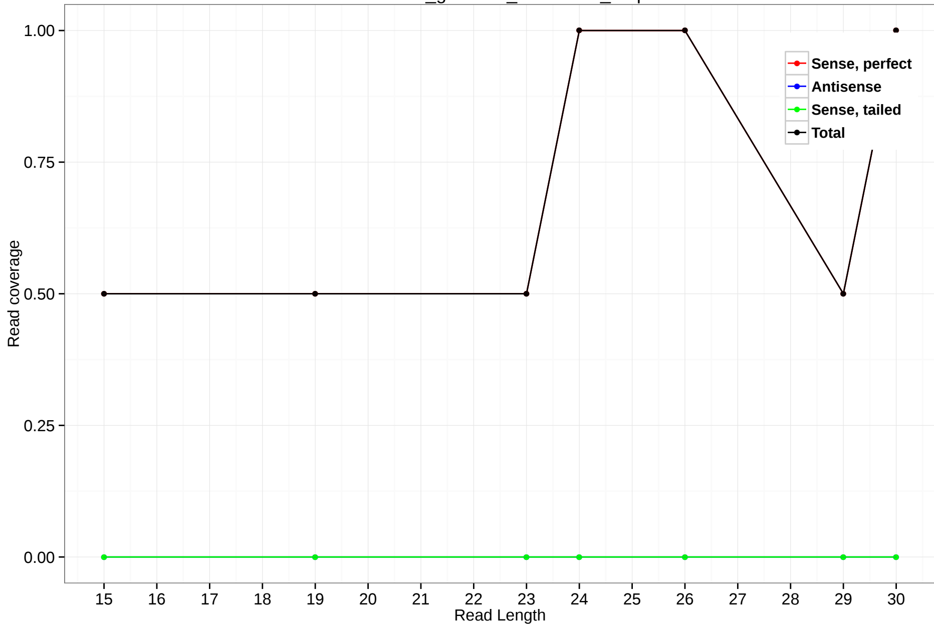
rheMac3_genscan_chr2.1443_4.5p
