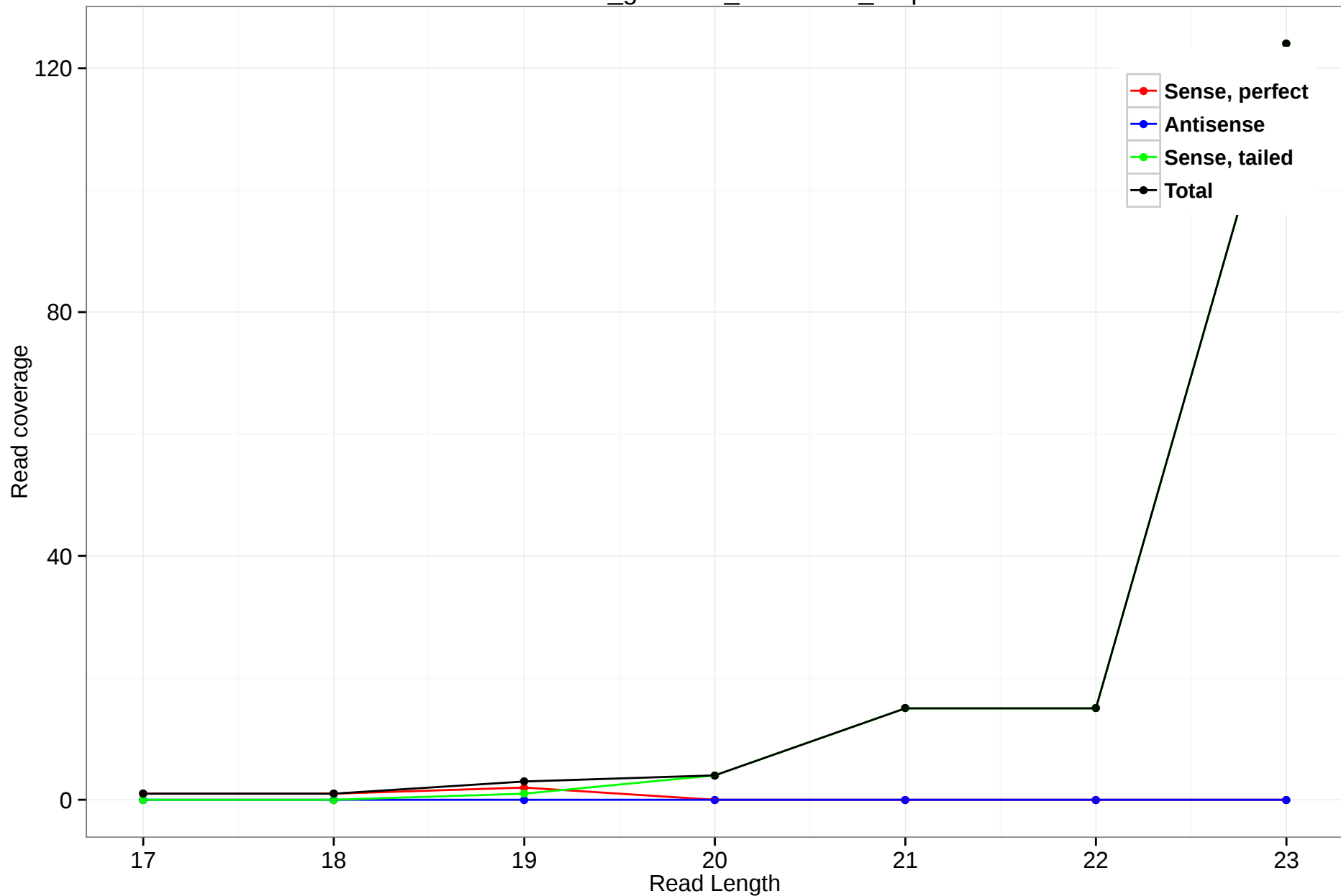
rheMac3_genscan_chr2.1427_1.3p
