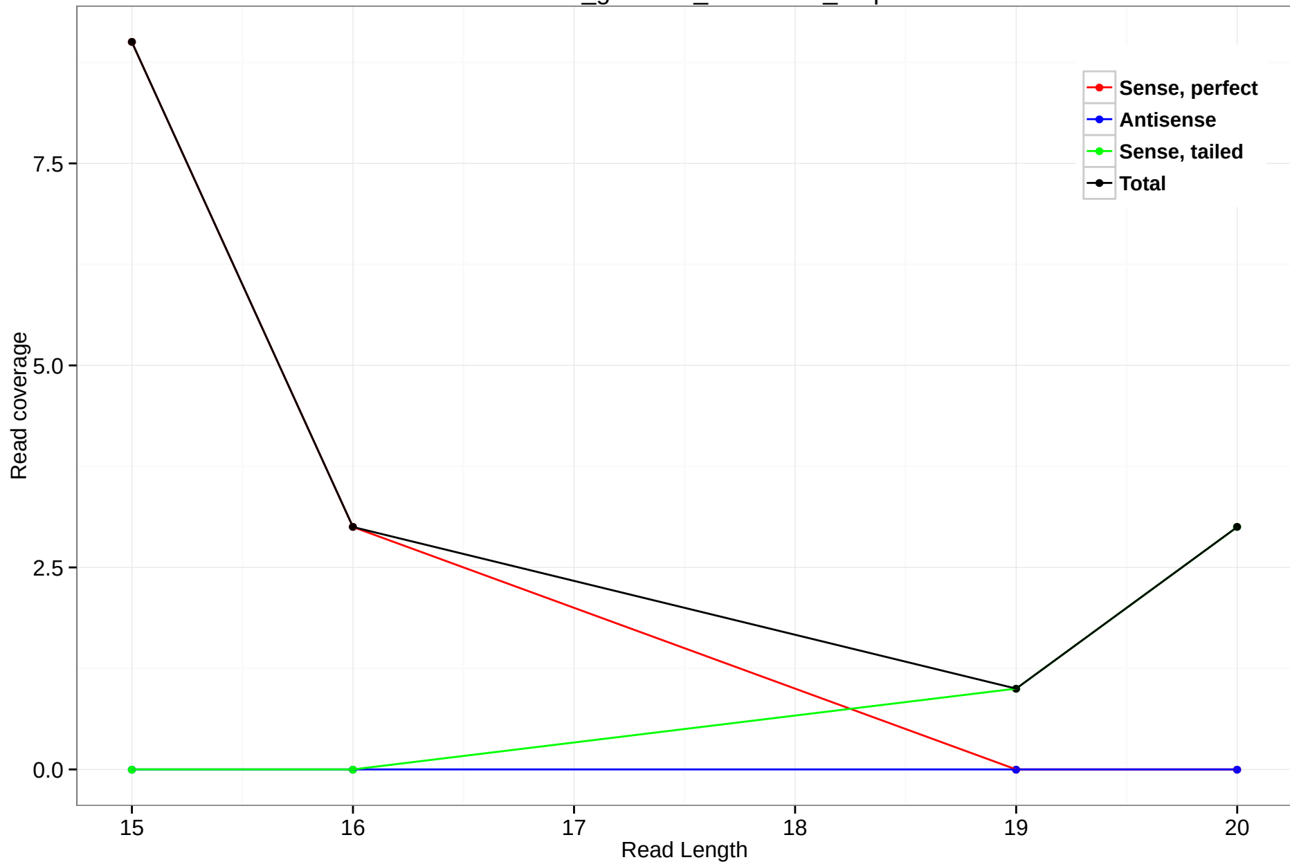
rheMac3_genscan_chr2.1417_8.3p
