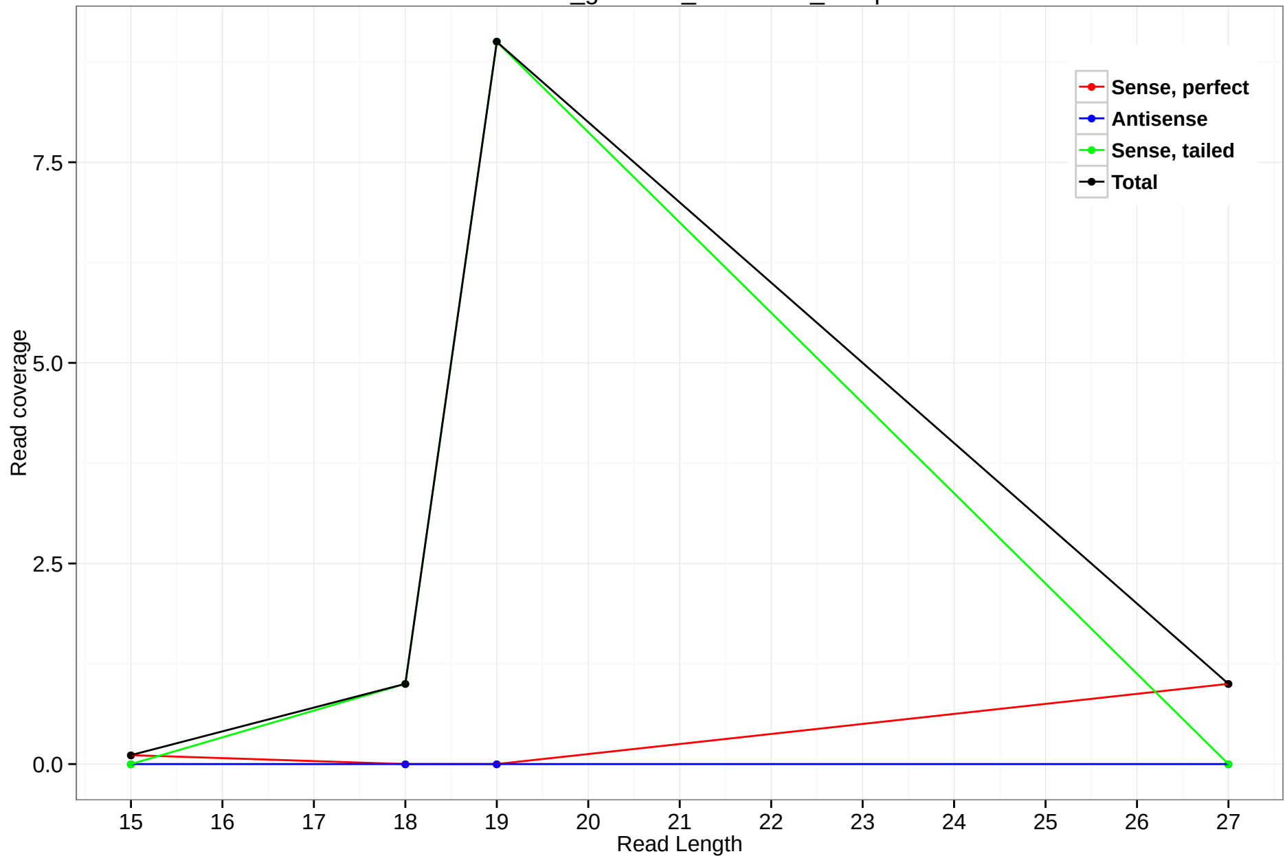
rheMac3_genscan_chr2.1251_42.3p
