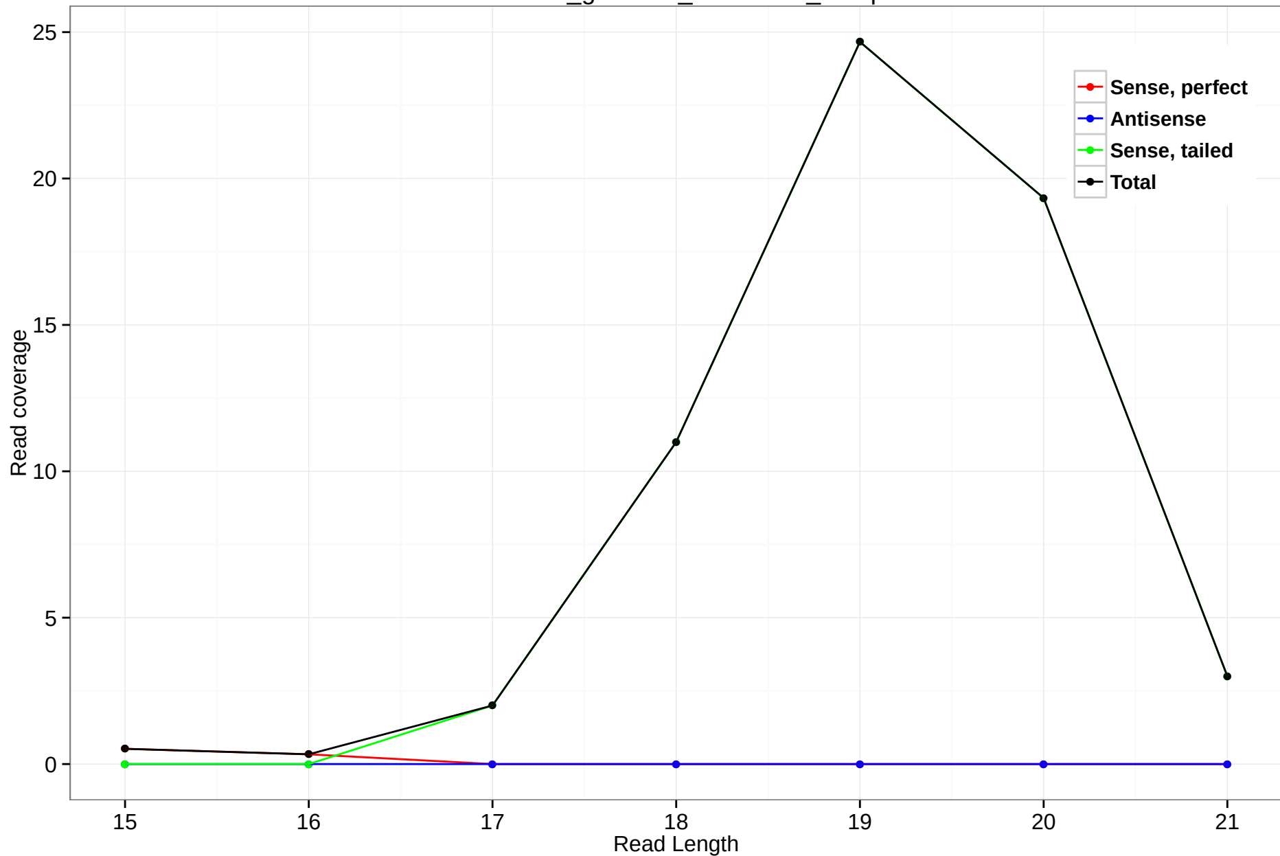
rheMac3_genscan_chr2.1225_10.3p
