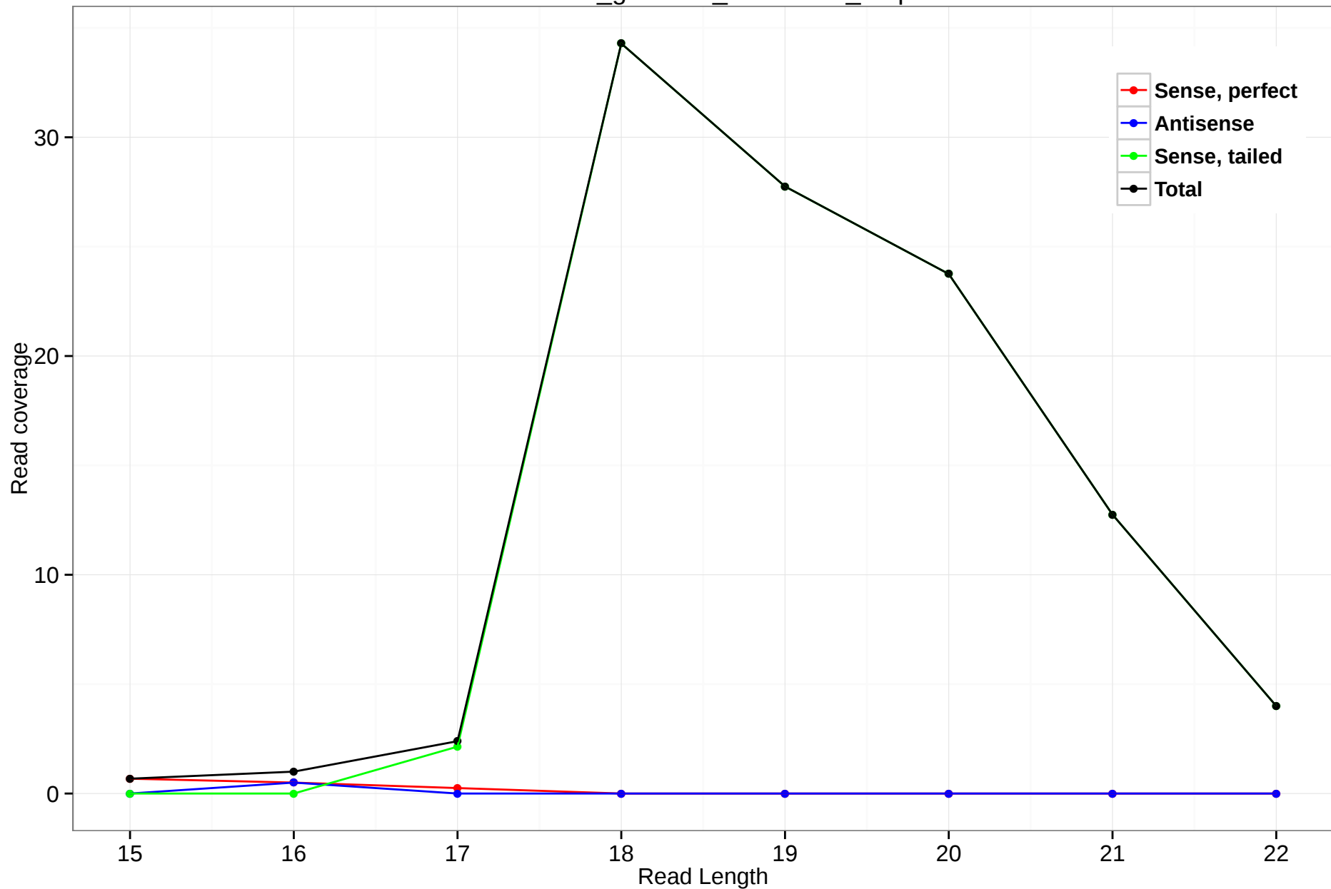
rheMac3_genscan_chr2.1220_5.3p
