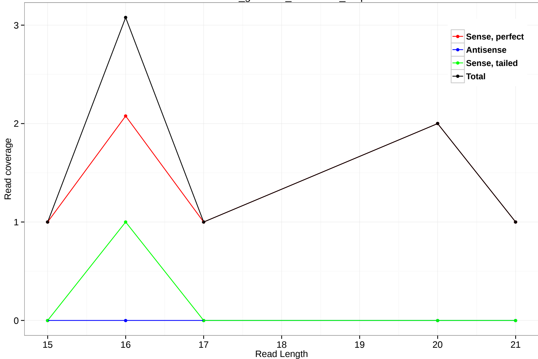
rheMac3_genscan_chr2.1063_2.5p
