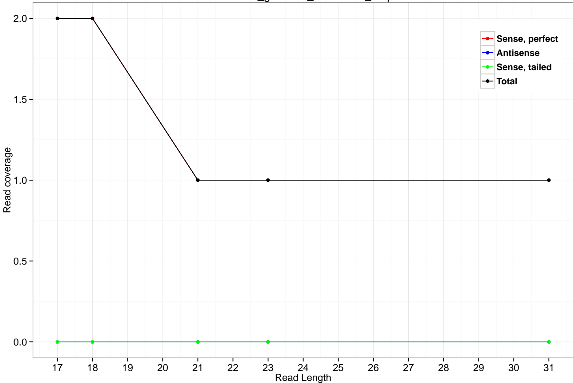
rheMac3_genscan_chr2.1033_2.3p
