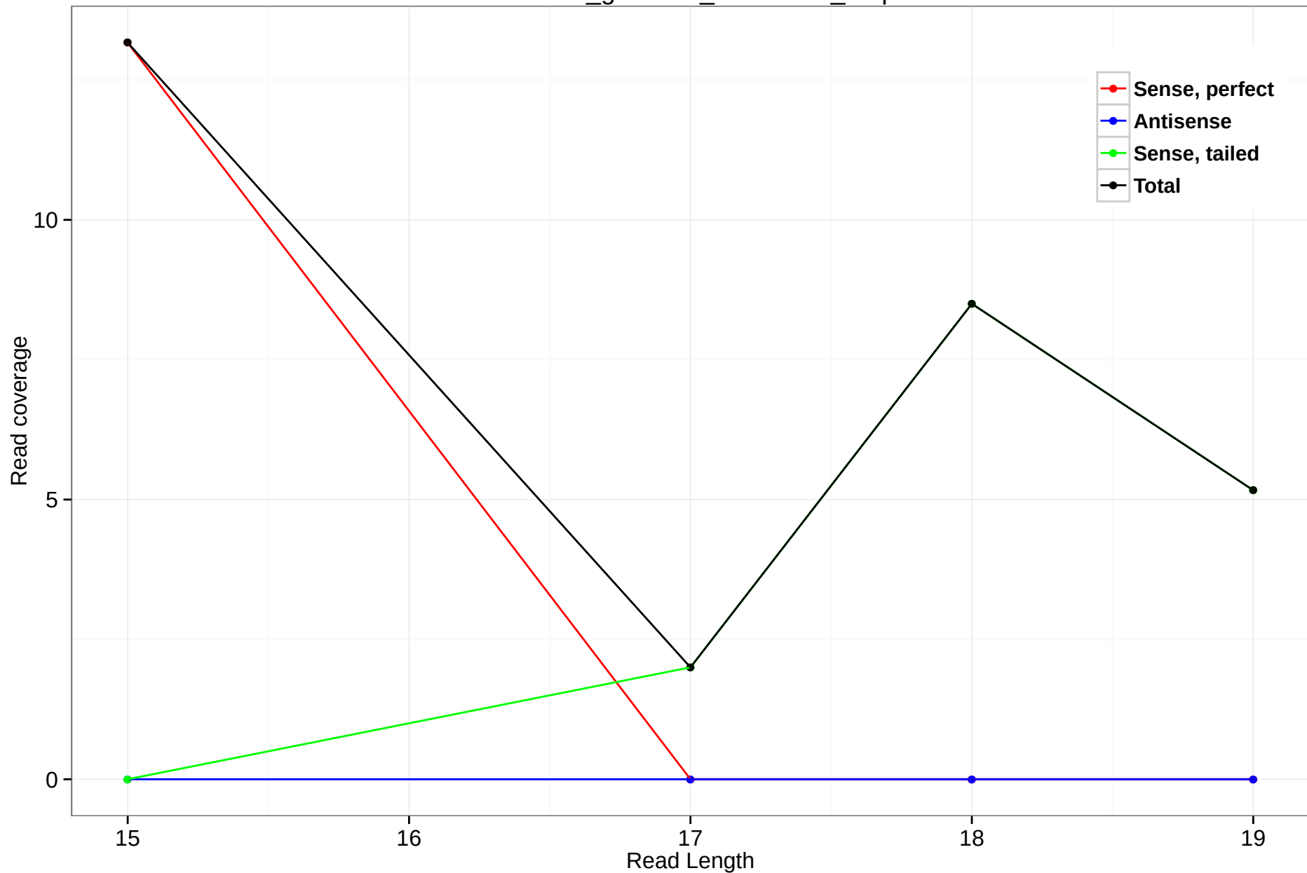
rheMac3_genscan_chr15.994_8.3p
