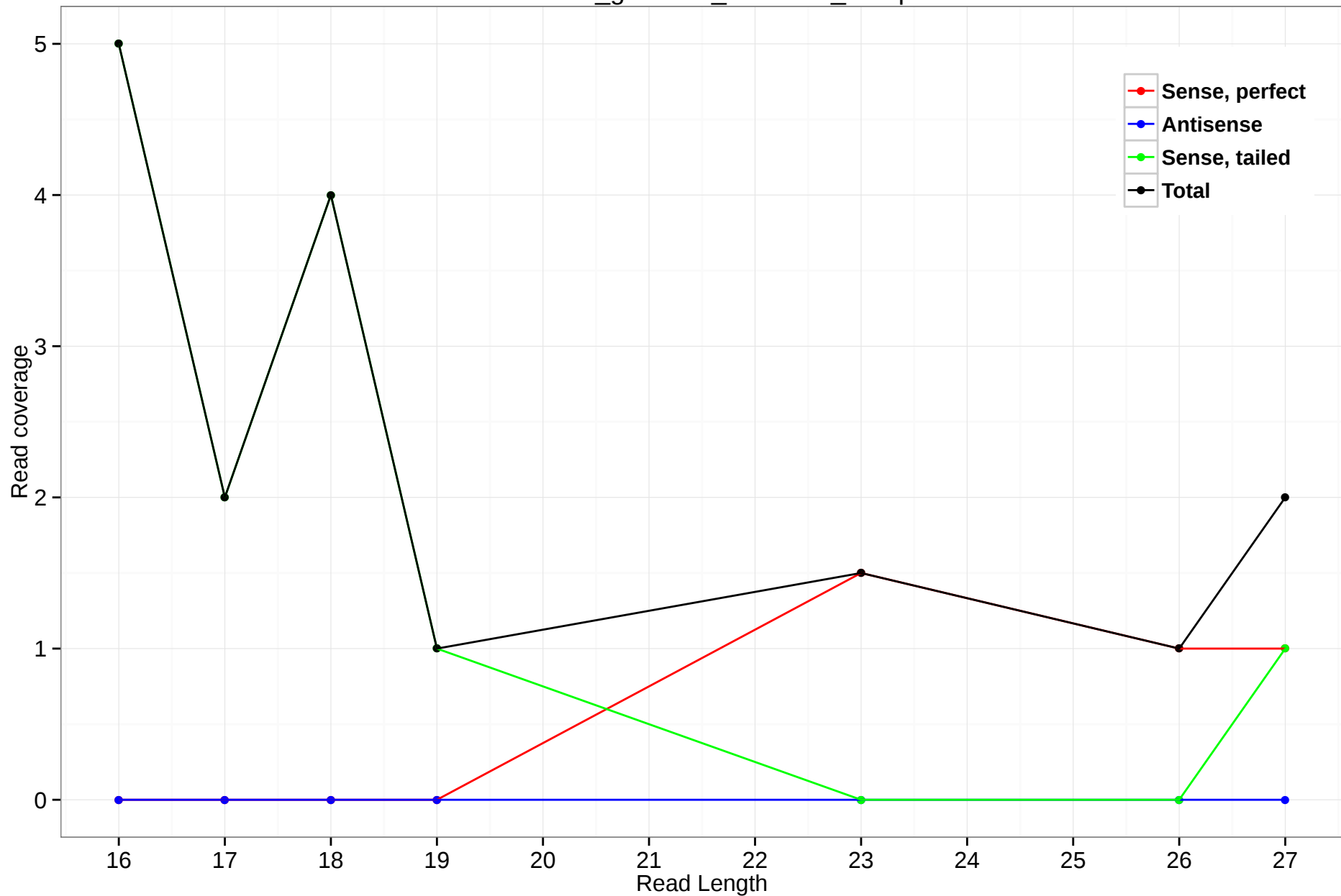
rheMac3_genscan_chr15.94_10.3p
