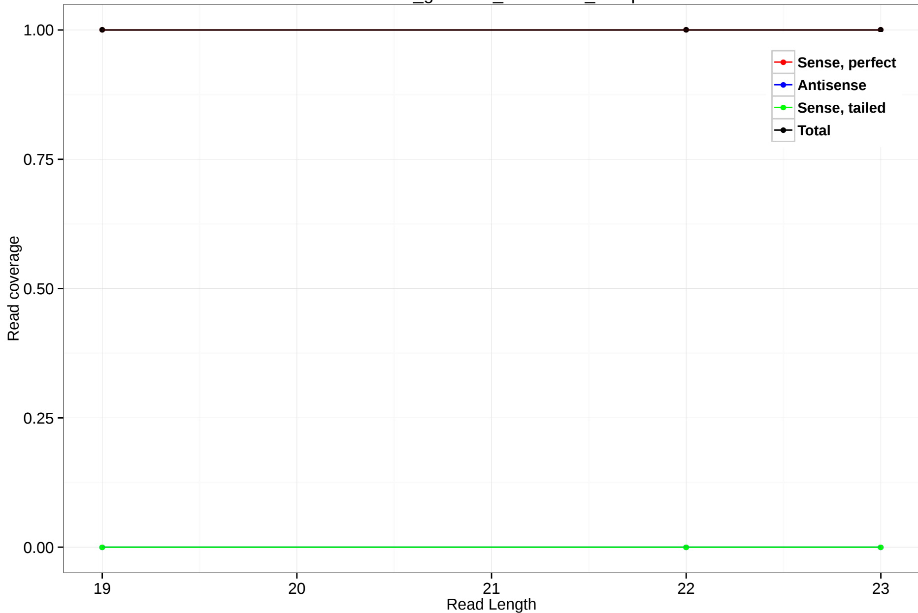
rheMac3_genscan_chr15.892_28.3p
