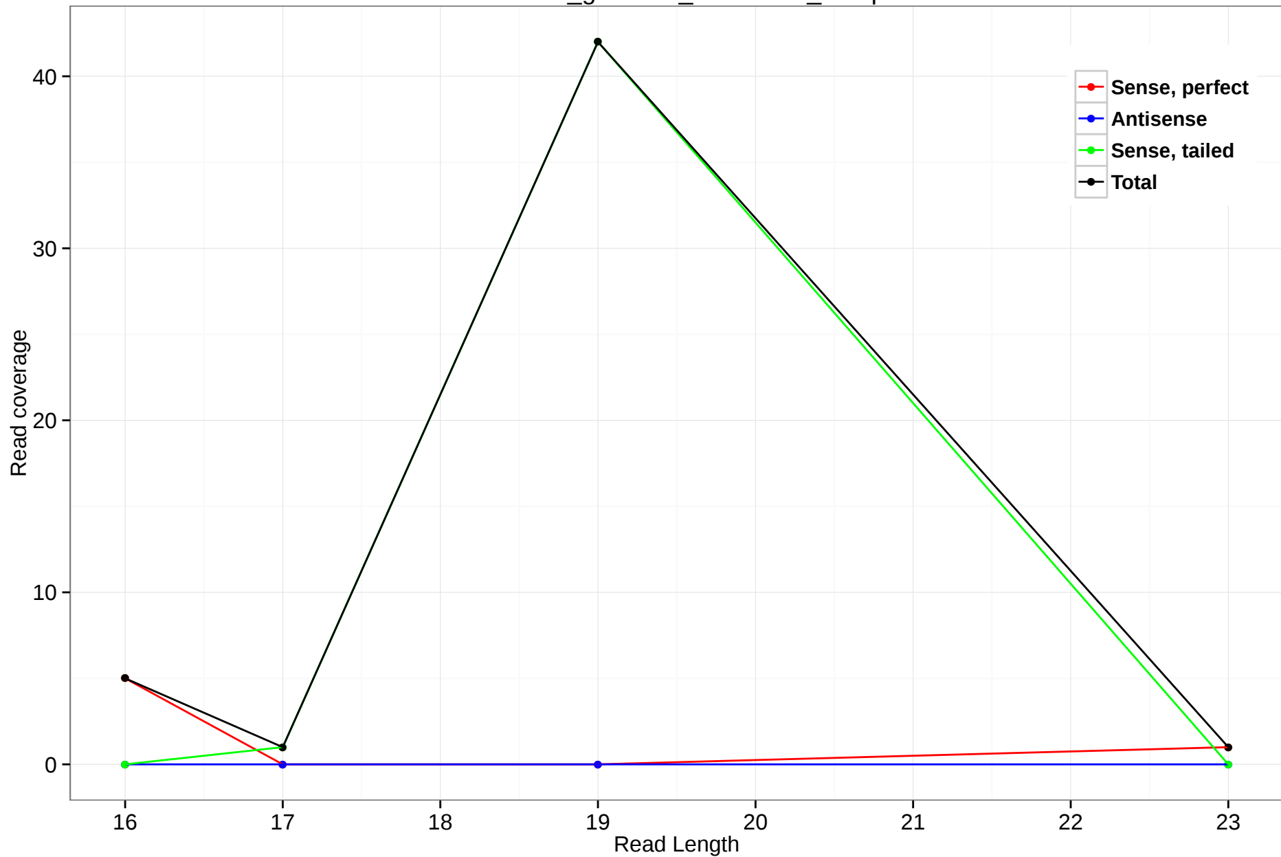
rheMac3_genscan_chr15.886_19.3p
