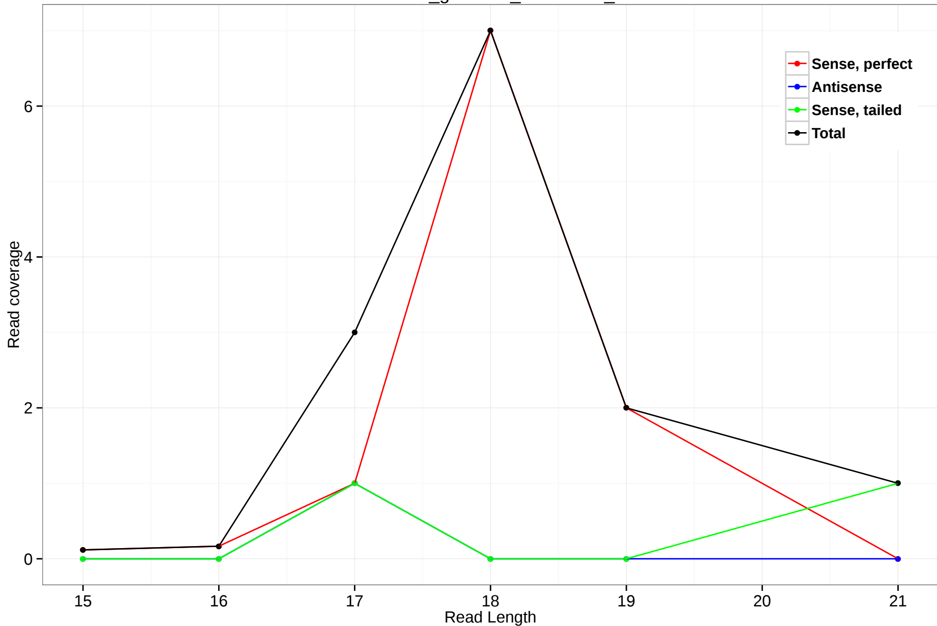
rheMac3_genscan_chr15.678_2
