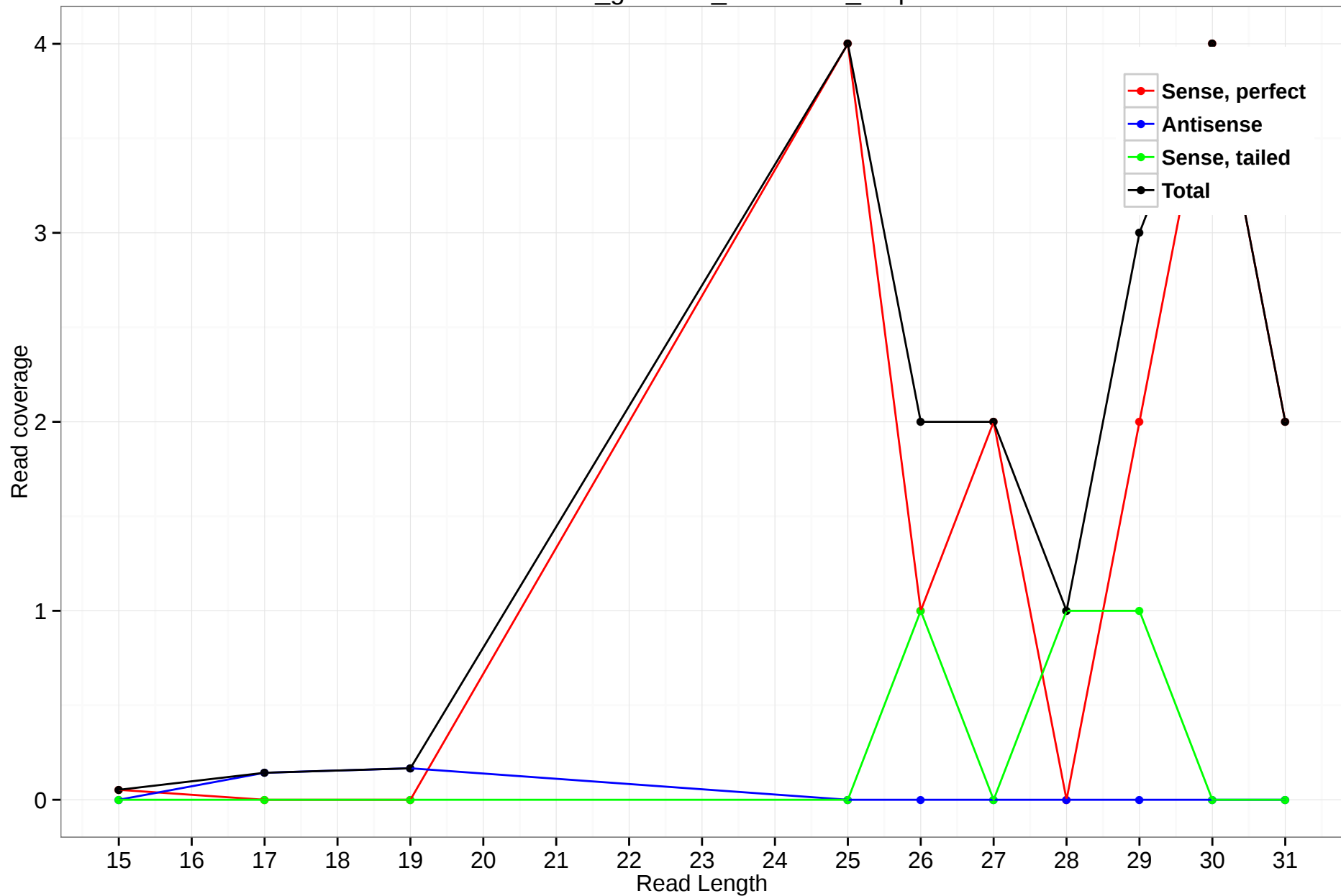
rheMac3_genscan_chr15.659_7.3p
