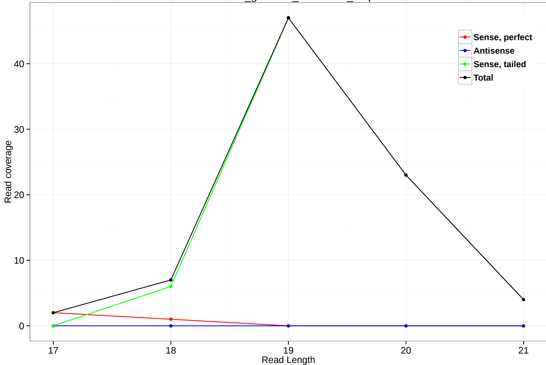
rheMac3_genscan_chr15.534_1.5p
