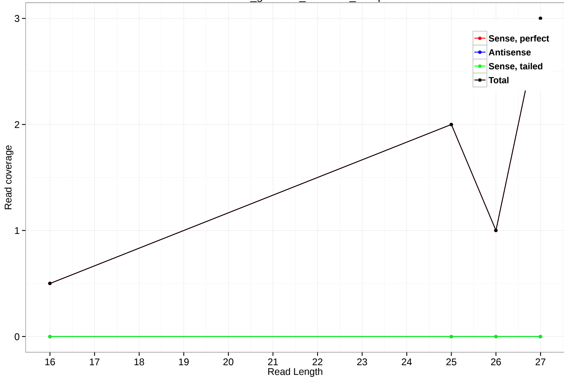
rheMac3_genscan_chr15.51_12.3p
