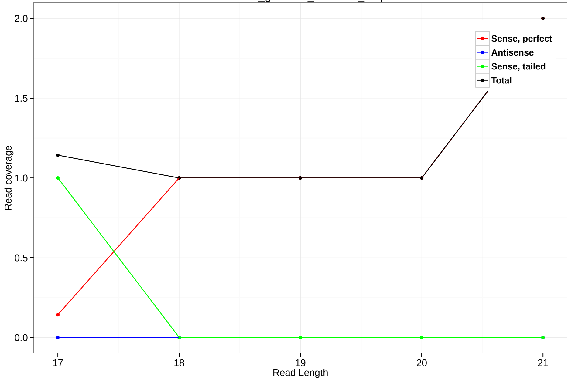
rheMac3_genscan_chr15.49_1.5p
