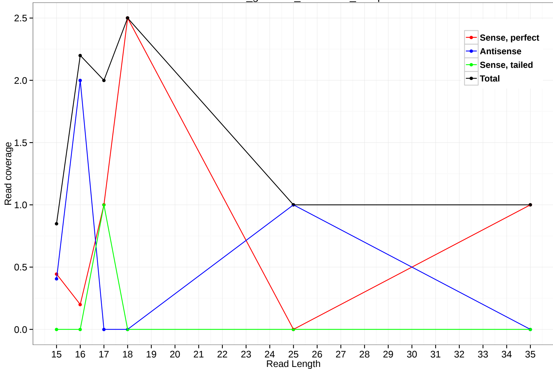
rheMac3_genscan_chr15.455_35.5p
