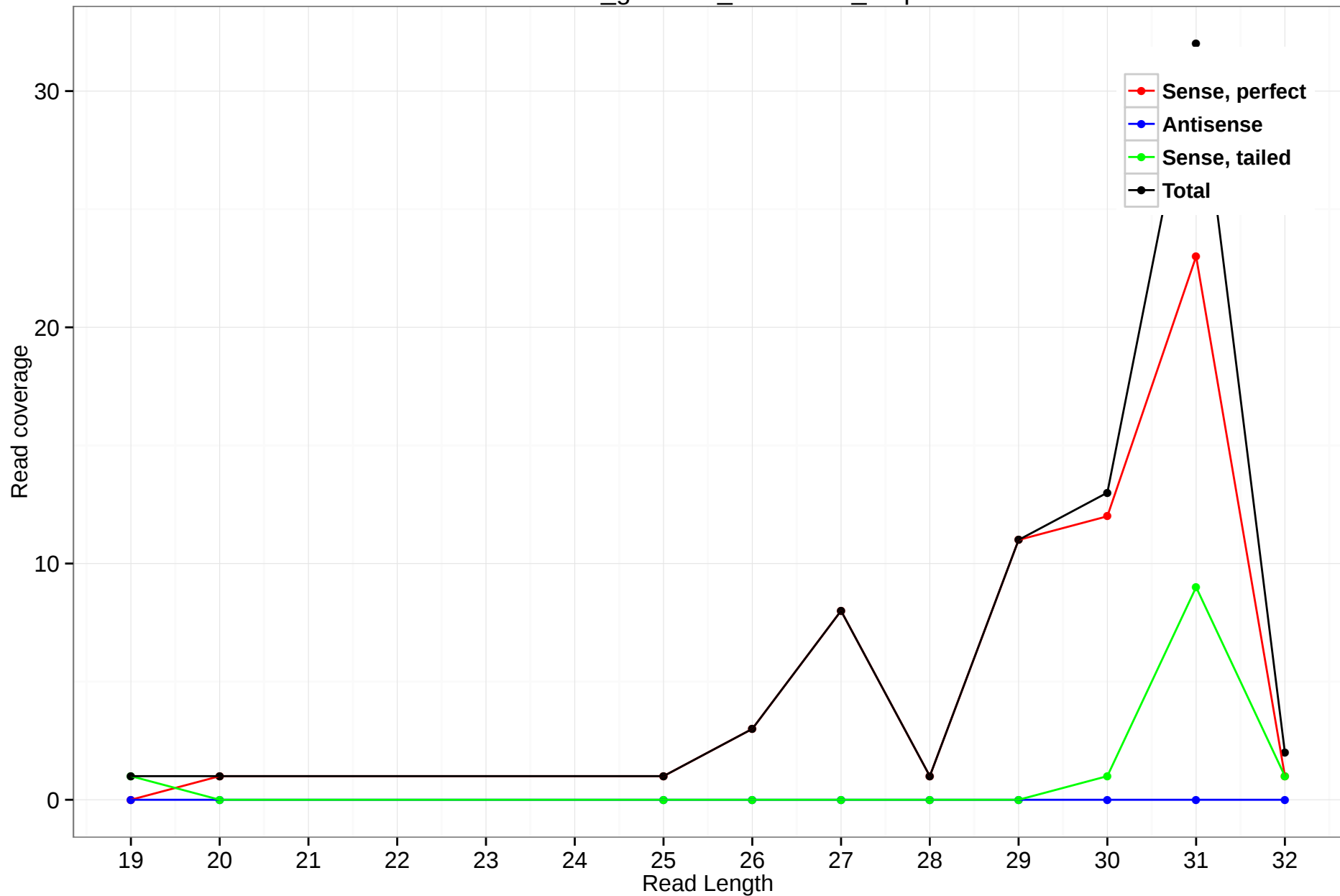
rheMac3_genscan_chr15.434_6.3p
