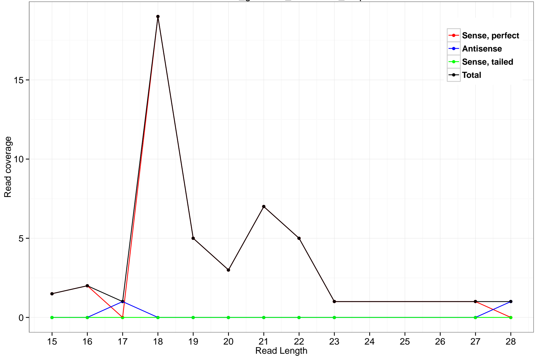
rheMac3_genscan_chr15.400_2.5p
