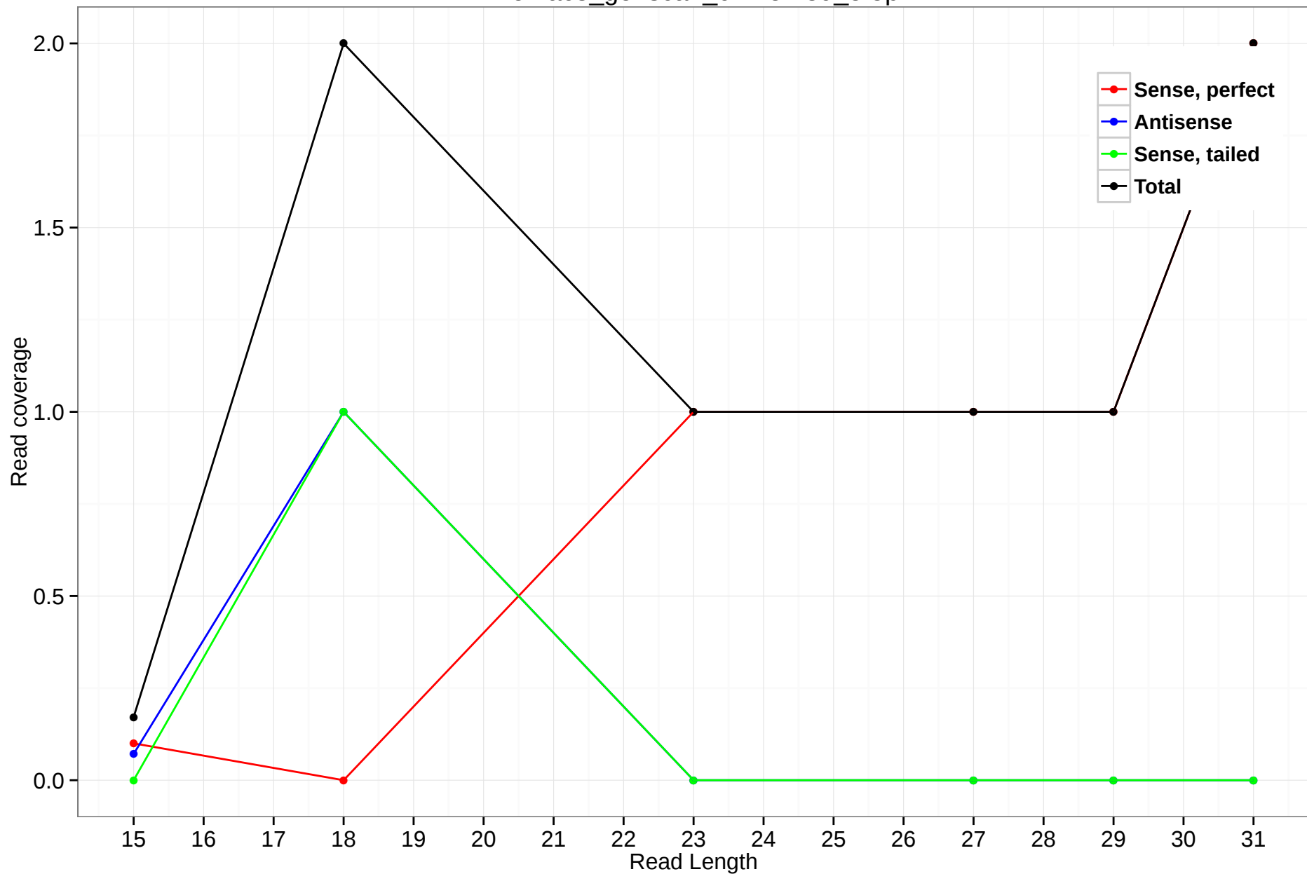
rheMac3_genscan_chr15.289_5.5p
