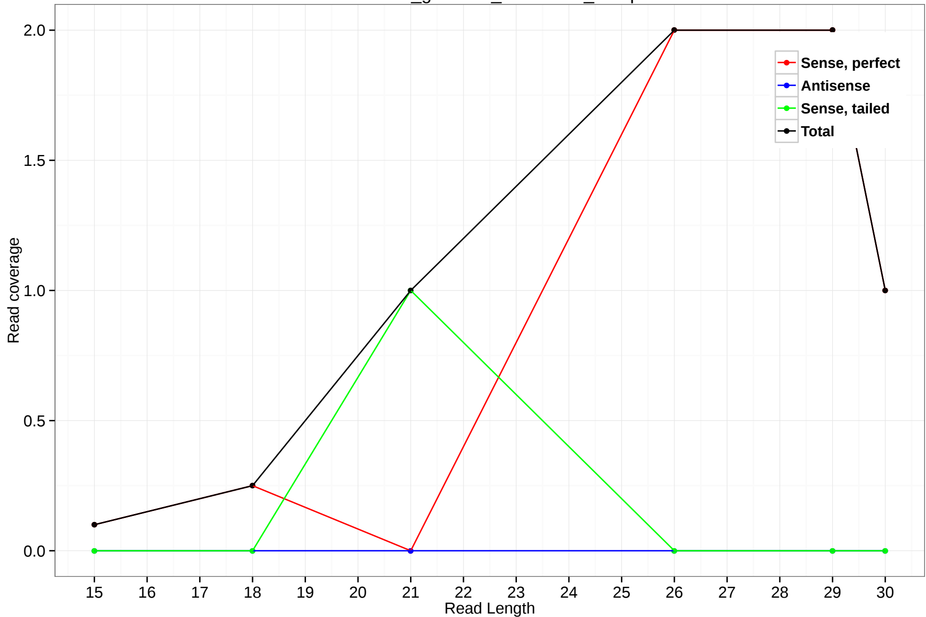
rheMac3_genscan_chr15.283_24.5p
