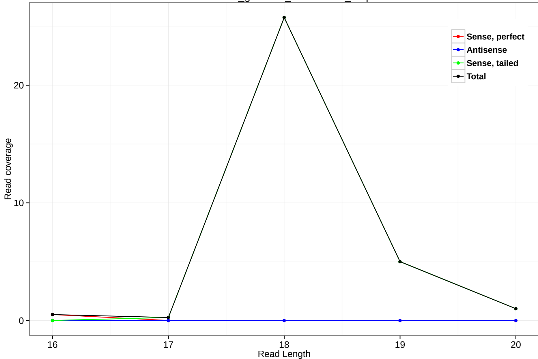
rheMac3_genscan_chr15.2265_3.5p
