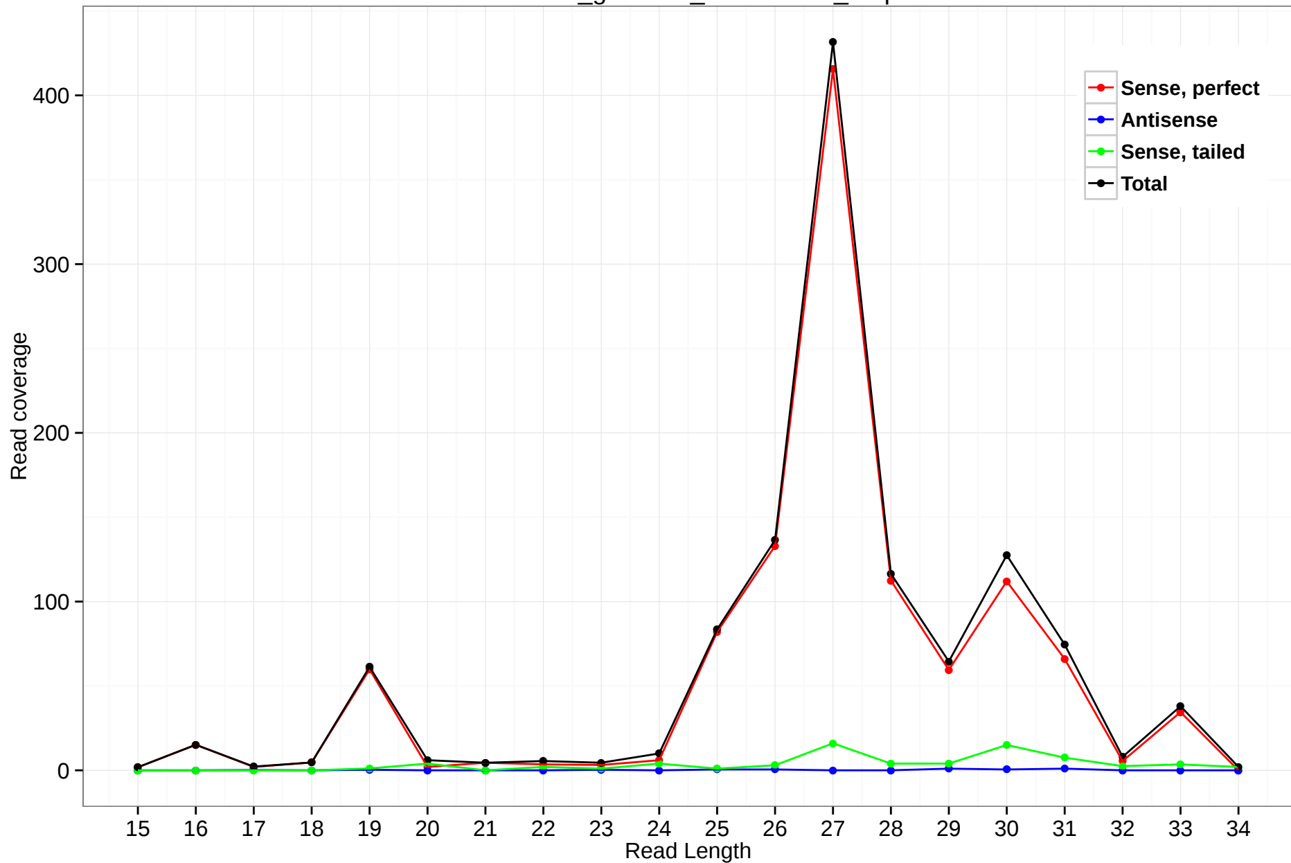
rheMac3_genscan_chr15.2247_7.5p
