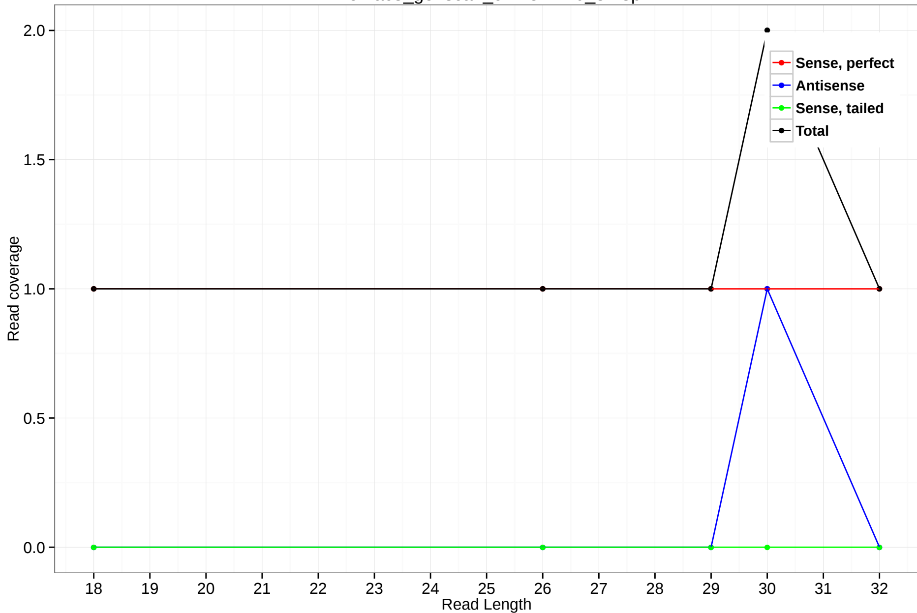
rheMac3_genscan_chr15.2170_34.3p
