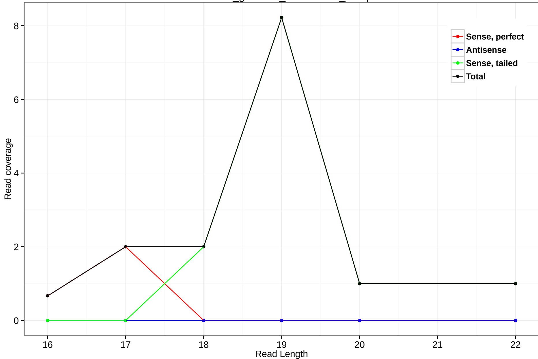
rheMac3_genscan_chr15.2170_29.5p
