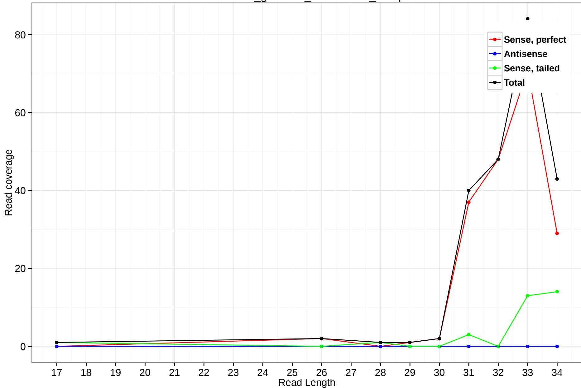
rheMac3_genscan_chr15.2170_12.5p
