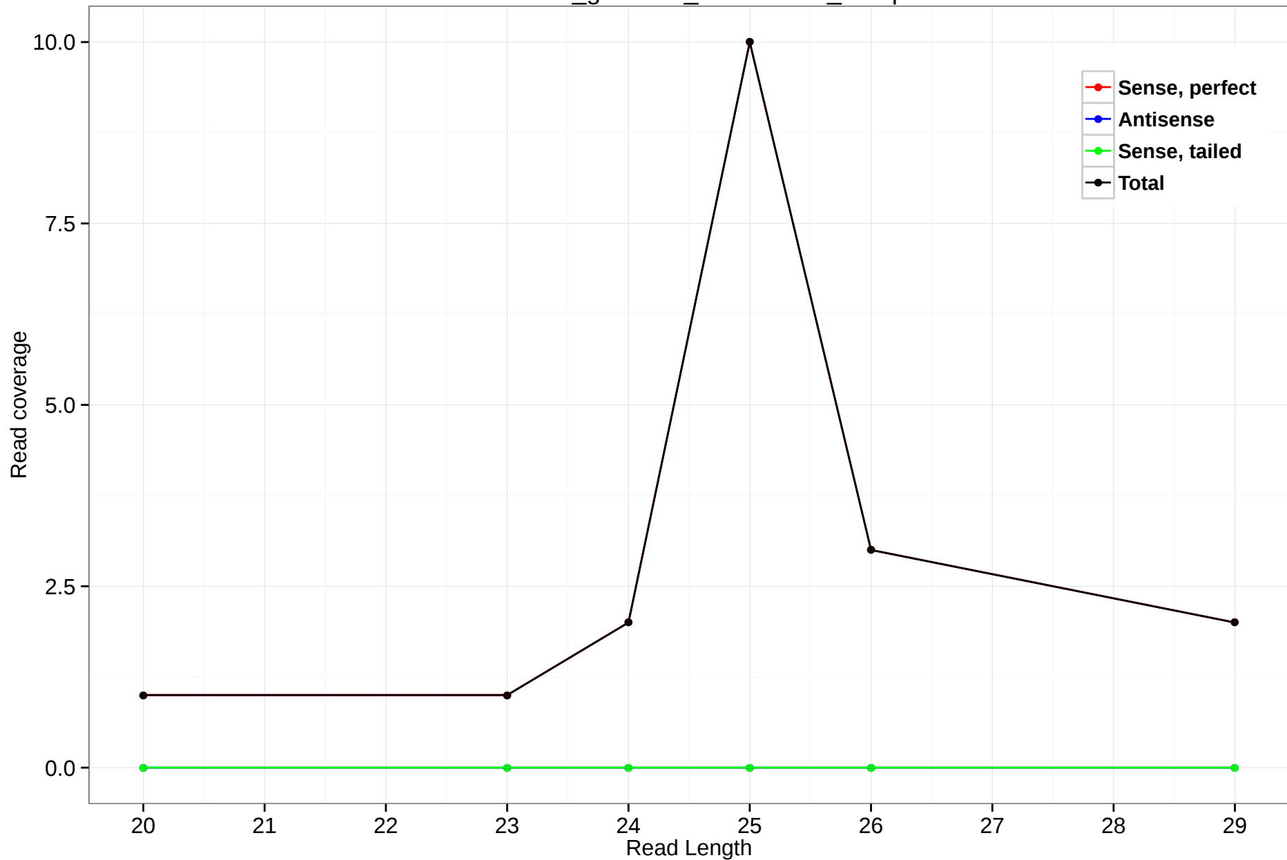
rheMac3_genscan_chr15.2167_12.5p
