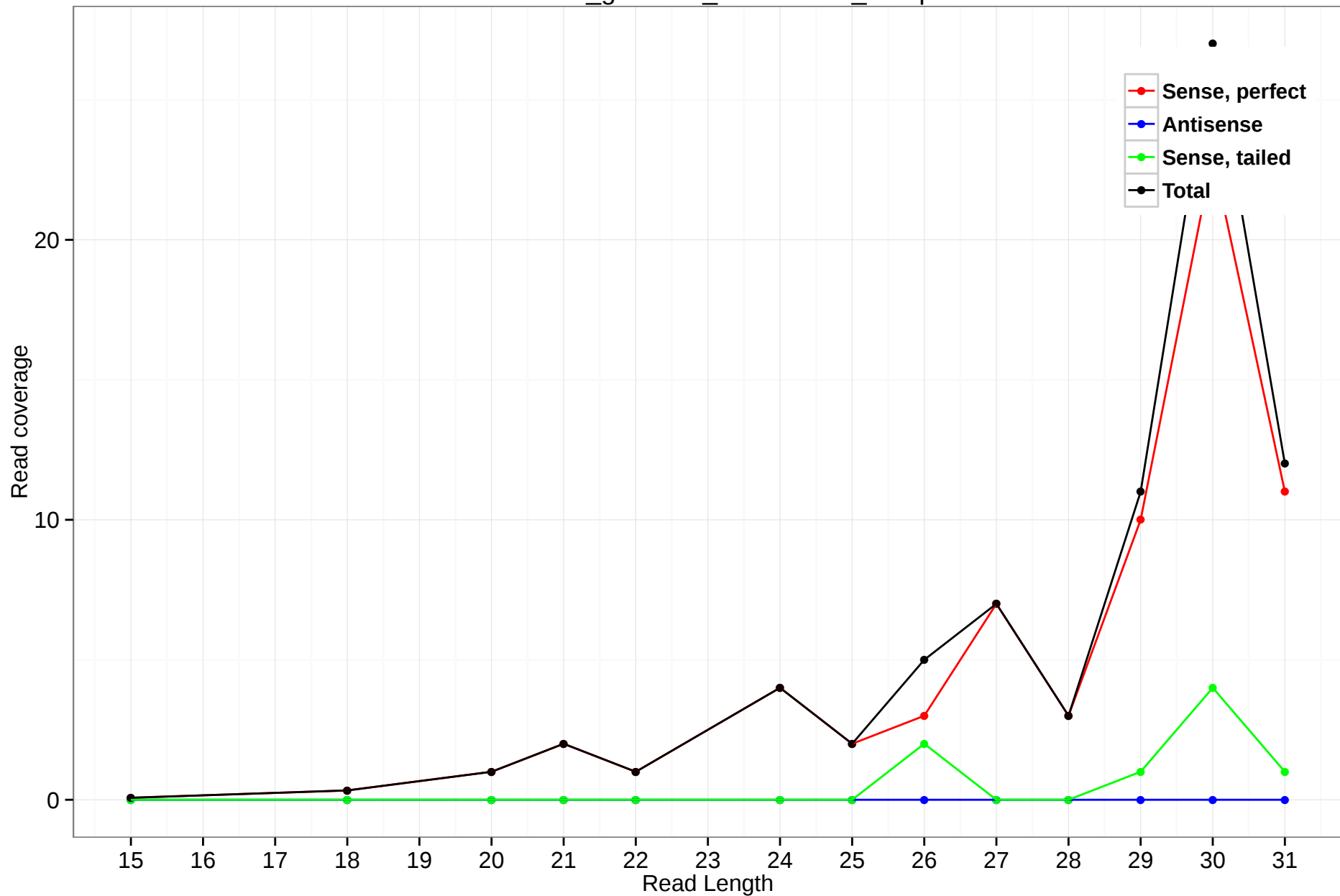
rheMac3_genscan_chr15.2167_12.3p
