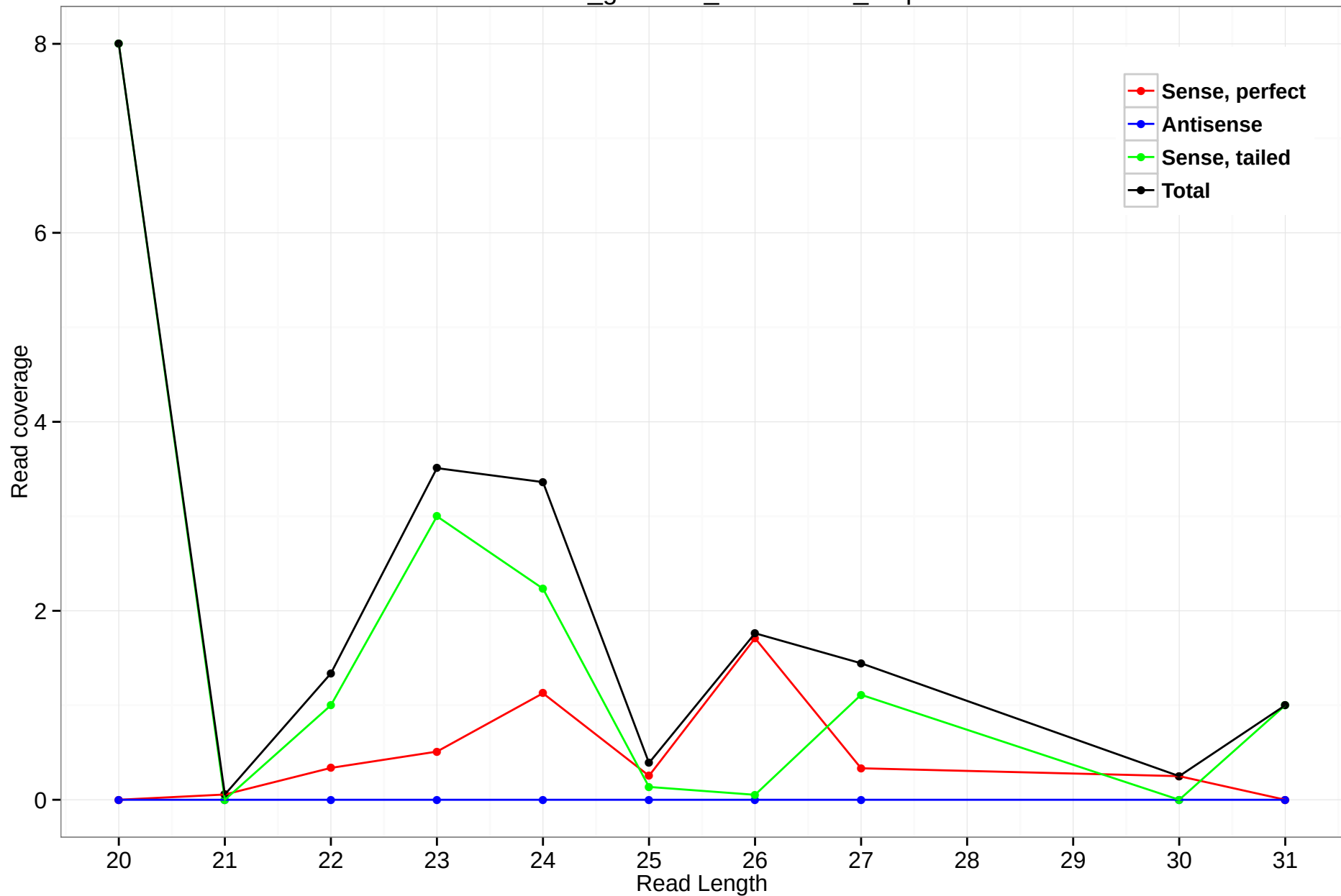
rheMac3_genscan_chr15.2165_0.3p
