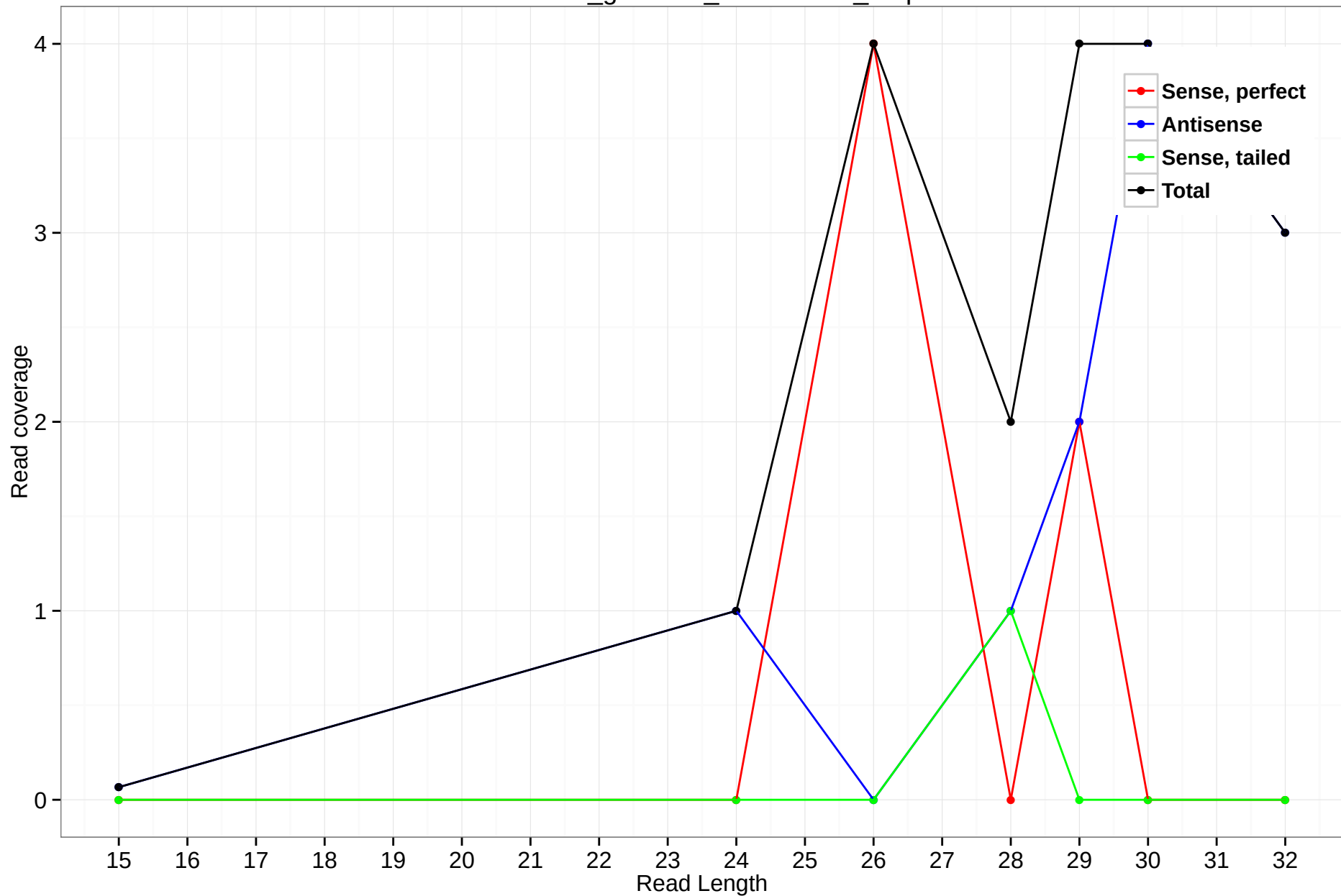
rheMac3_genscan_chr15.2091_5.3p
