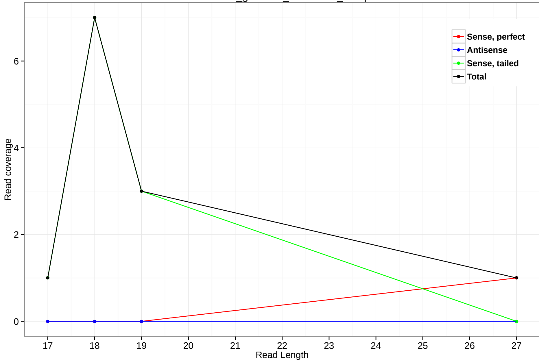
rheMac3_genscan_chr15.204_13.5p
