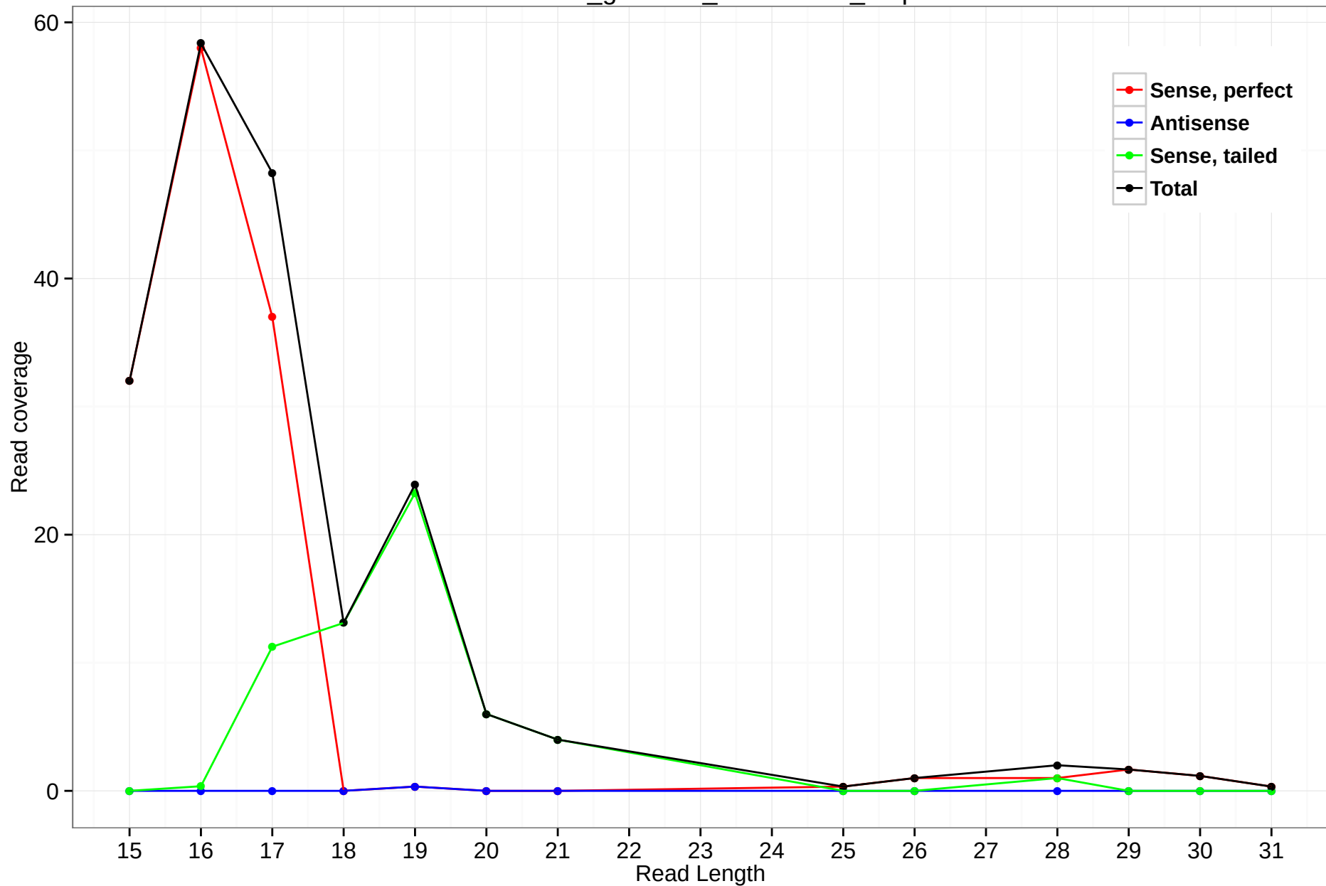
rheMac3_genscan_chr15.1978_4.5p
